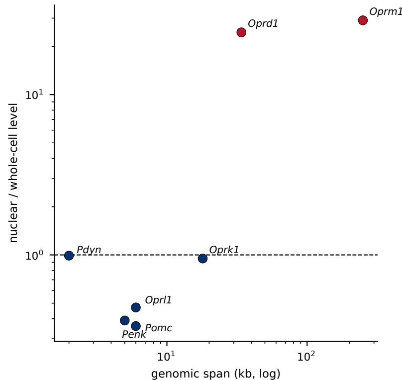
(B) The inversion tracks gene length same tissue, log-log r = 0.84 ( n = 7 )
