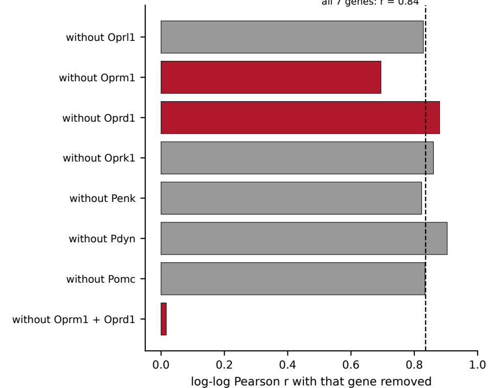
(C) Two genes carry the correlation r = 0.02 without both all 7 genes: r = 0.84
