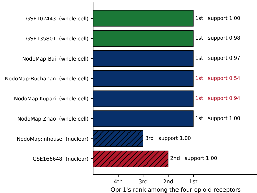
(A) Oprl1 leads in every whole-cell dataset hatched = nuclear prep; red = bootstrap support < 0.95
