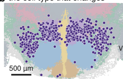
b the cell type that changes
