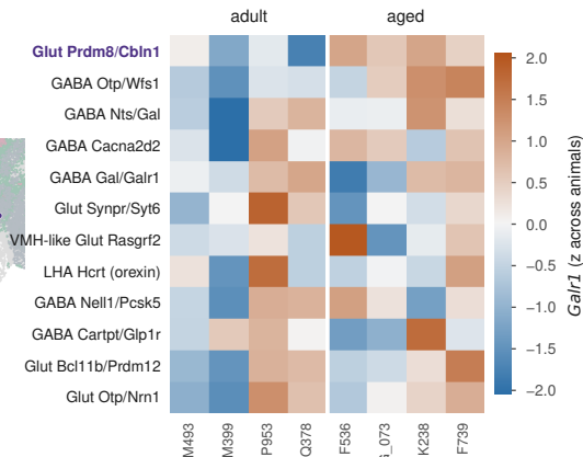
b the cell type that changes
