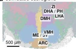
a delineated subregions
