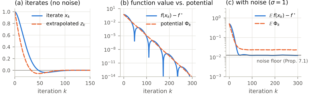
Figure 1: Heavy ball on f(x) = \frac{1}{2}x^2 ( L = 1 ) with \beta = 0.9 and \alpha = (1 - \beta)^2/(2L) = 0.005 , the largest step allowed by Theorem 5.3(b) . (a) Without noise: the iterate x_k and the extrapolated point z_k , which moves ahead of x_k . (b) Without noise: f(x_k) - f^* is not monotone (it rises after each overshoot), while the potential \Phi_k of Theorem 5.3 decreases at every step. (c) With noise ( \sigma = 1 , average over 20 000 runs): both expectations settle at a noise floor; the floor of \mathbb{E}f(x_k) agrees with the exact value of Proposition 7.1 (horizontal line).
