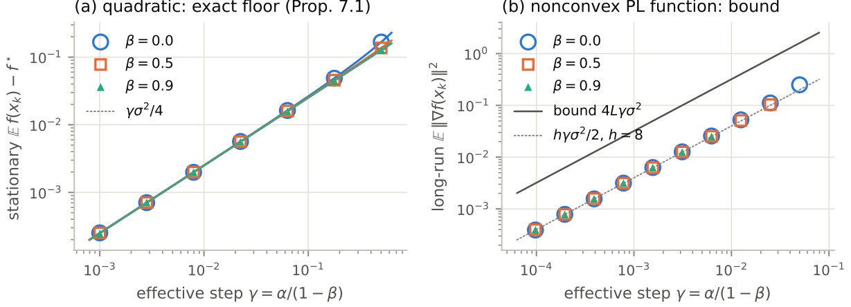
Figure 5: The noise floor with a constant step scales like \gamma\sigma^2 and, to first order, depends on (\alpha, \beta) only through \gamma (markers for different \beta lie on top of each other). (a) Quadratic (P1), \sigma = 1 : empirical stationary \mathbb{E}f(x_k) (markers; 4000 runs) and the exact formula (7.1) (lines). (b) Nonconvex PL function (P2), \sigma = 1 : long-run \mathbb{E}\|\nabla f(x_k)\|^2 (400 runs) for step sizes inside the range of Theorem 5.3, the bound 4L\gamma\sigma^2 of Theorem 6.1 (as K \rightarrow \infty ), and the local quadratic prediction h\gamma\sigma^2/2 with h = f''(0) = 8 .
