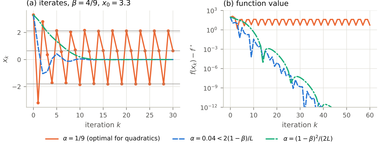
Figure 2: Heavy ball on the strongly convex function of Example 7.5 , \beta = \frac{4}{9} , x_{-1} = x_0 = 3.3 , exact gradients. (a) With the quadratic-optimal \alpha = \frac{1}{9} the iterates are attracted to the 3-cycle \{p_1, p_2, p_3\} (grey lines). (b) The function value then oscillates forever, while the step sizes allowed by Proposition 7.3 ( \alpha = 0.04 ) and by Theorem 5.3 ( \alpha = (1 - \beta)^2/(2L) ) converge.
