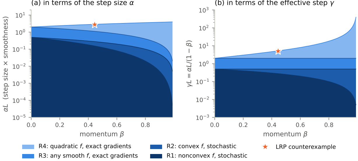
Figure 3: Where each guarantee holds. Nested regions of admissible parameters, (a) in terms of \alpha L , (b) in terms of the effective step \gamma L = \alpha L / (1 - \beta) (log scales). R1: Theorem 5.3 (nonconvex, stochastic); R2: Theorem 6.8 (convex, stochastic); R3: Proposition 7.3 (any smooth f , exact gradients); R4: Proposition 7.2 (quadratics, exact gradients). The star marks the parameters of Example 7.5 , for which heavy ball cycles on a strongly convex function.
