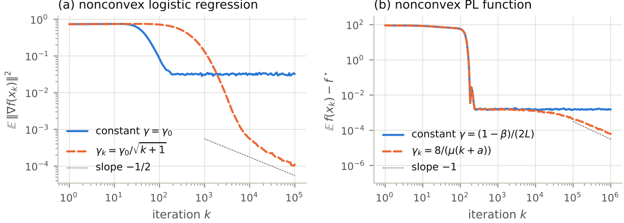
Figure 6: Diminishing step sizes remove the noise floor ( \beta = 0.9 ; both schedules start from the same \gamma_0 = \frac{1-\beta}{2L} ). (a) Nonconvex logistic regression (P3), 50 runs: constant step versus \gamma_k = \gamma_0/\sqrt{k+1} (Theorem 6.4(c)). (b) Nonconvex PL function (P2), 100 runs: constant step versus \gamma_k = \frac{8}{\mu(k+a)} with a = \frac{16L}{\mu(1-\beta)} (Corollary 6.7); the dotted lines have slopes -\frac{1}{2} and -1 .
