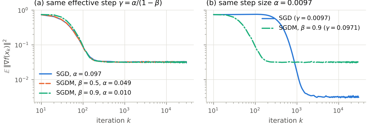
Figure 4: SGD versus SGDM on the nonconvex logistic regression problem (P3), mean of \|\nabla f(x_k)\|^2 over 100 runs (lightly smoothed). (a) Same effective step \gamma = \frac{1-0.9}{2L} , inside the range of Theorem 5.3 for every \beta shown: the three methods are indistinguishable. (b) Same raw step \alpha = \frac{(1-0.9)^2}{2L} : momentum \beta = 0.9 makes the effective step 10 times larger, so it converges faster at first but stalls at a 10 times higher noise floor.
