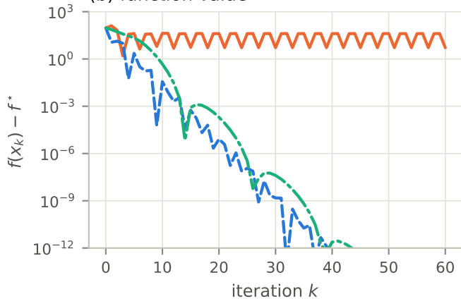
(b) function value
