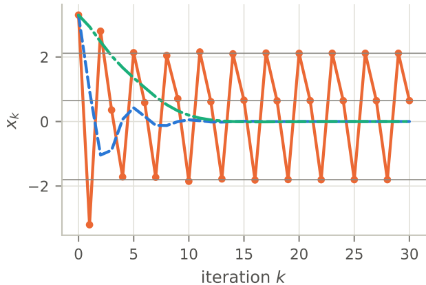
(a) iterates, \beta = 4/9 , x_0 = 3.3
