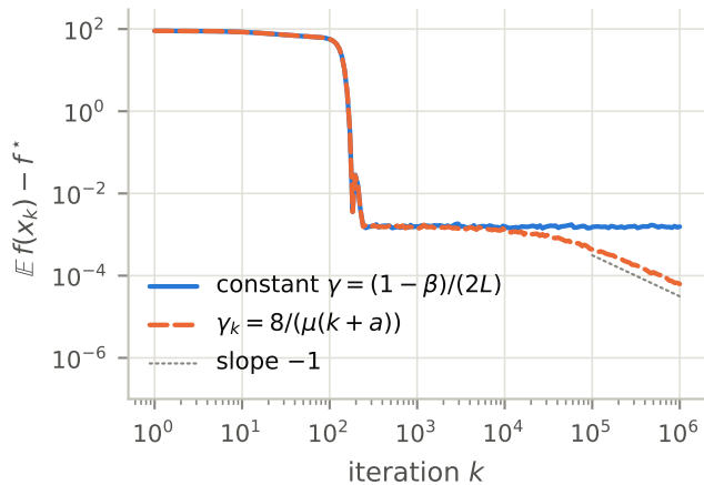
(b) nonconvex PL function
