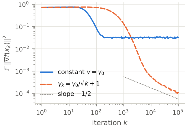
(a) nonconvex logistic regression
