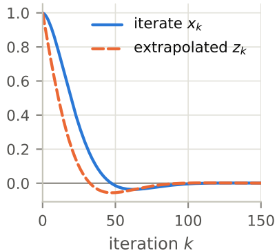
(a) iterates (no noise)
