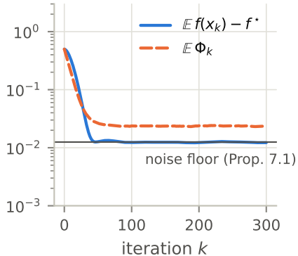
(c) with noise ( \sigma = 1 )
