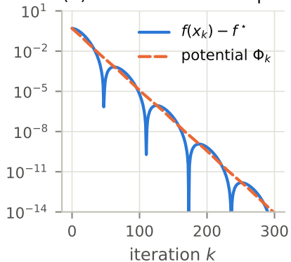
(b) function value vs. potential
