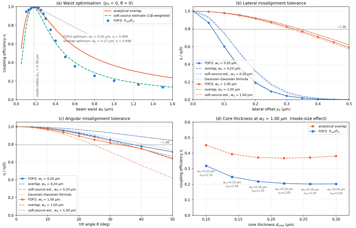
Figure A1. Beam-parameter sweeps on the untapered waveguide: waist, lateral offset, tilt and core thickness.
