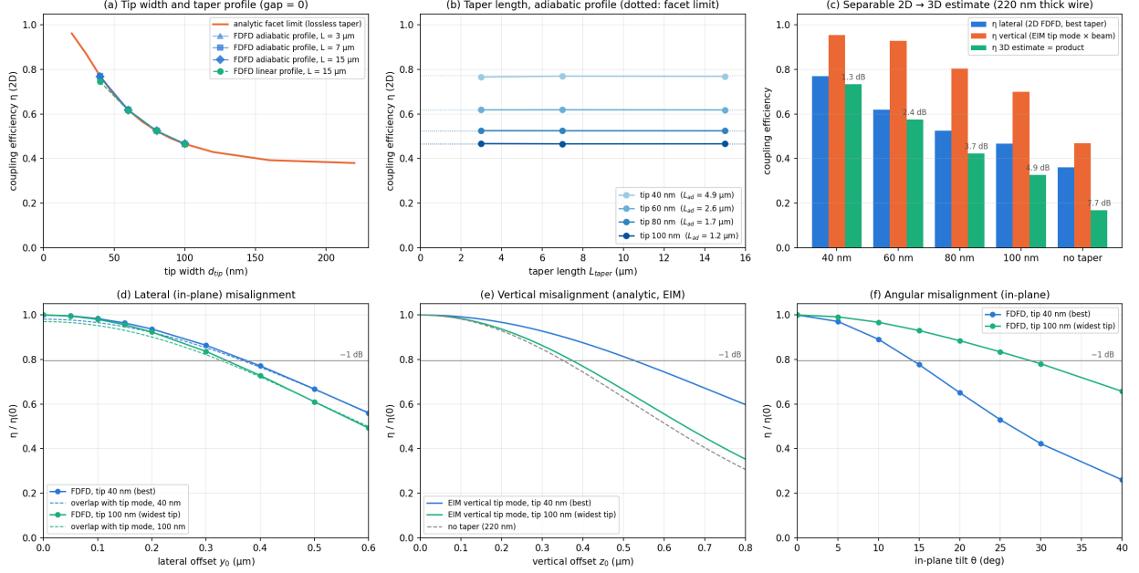
Figure 4. Design study (fddf_coupler_design.py): (a) tip width and profile; (b) taper length per tip with the analytic facet limits; (c) separable 2D → 3D estimate; (d) lateral, (e) vertical and (f) angular misalignment tolerance.
