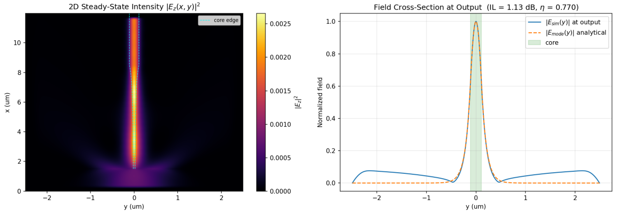
Figure 5. Field of the final design (40 nm tip, adiabatic taper, 7 μm, gap 0).
