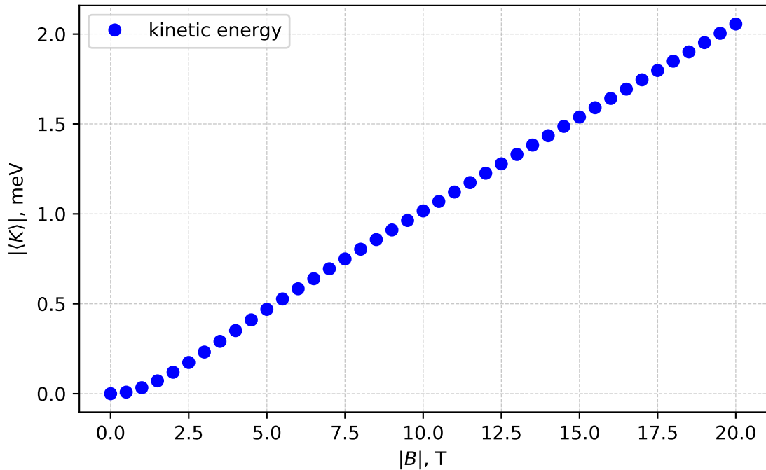
Kinetic energy at T = 2.0 K
