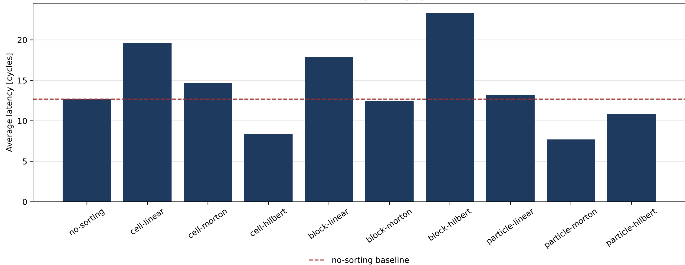
Force Traversal Memory Latency by Variant
