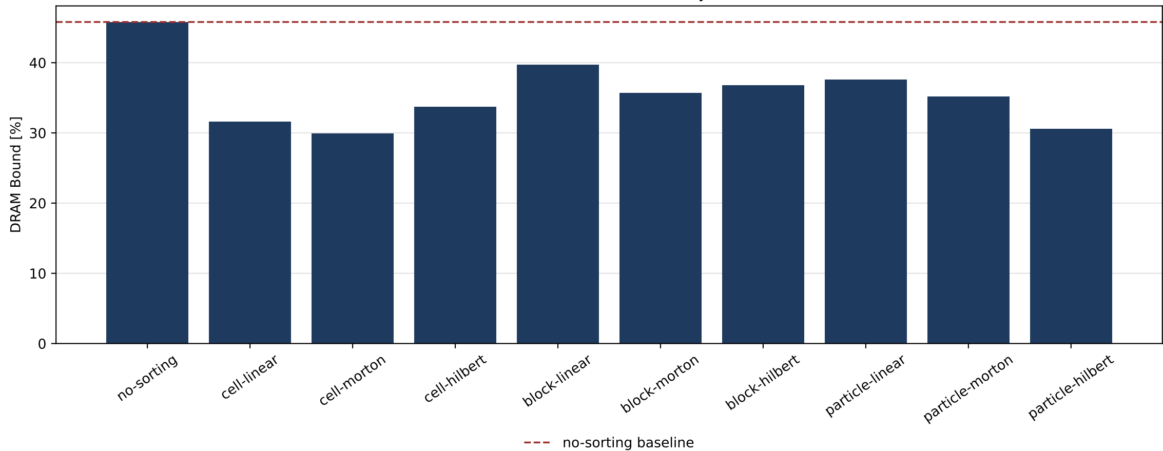
Force Traversal DRAM Bound by Variant
