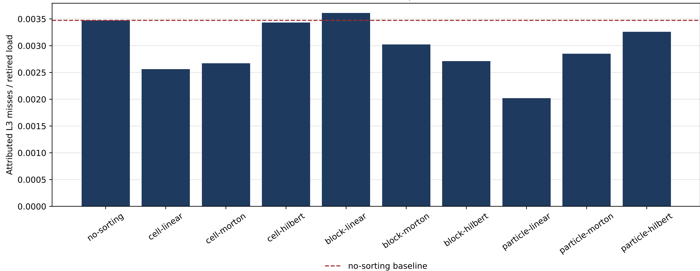
Whole-Run L3 Misses per Load
