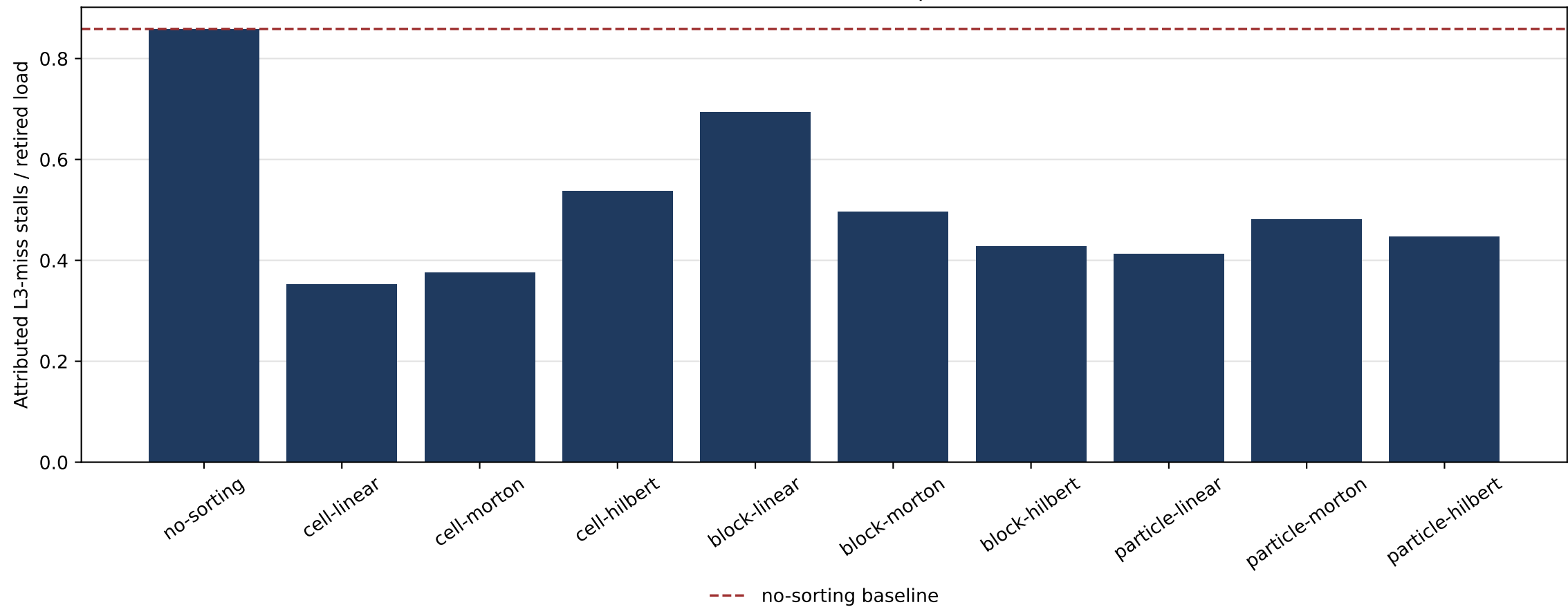
Whole-Run L3-Miss Stalls per Load
