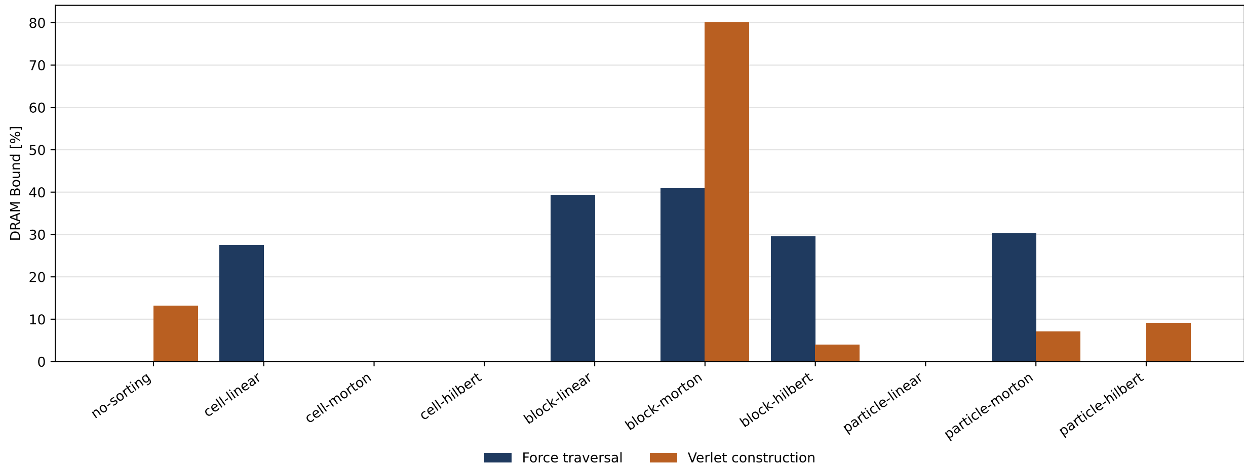
DRAM Bound in Main Particle-Access Phases
