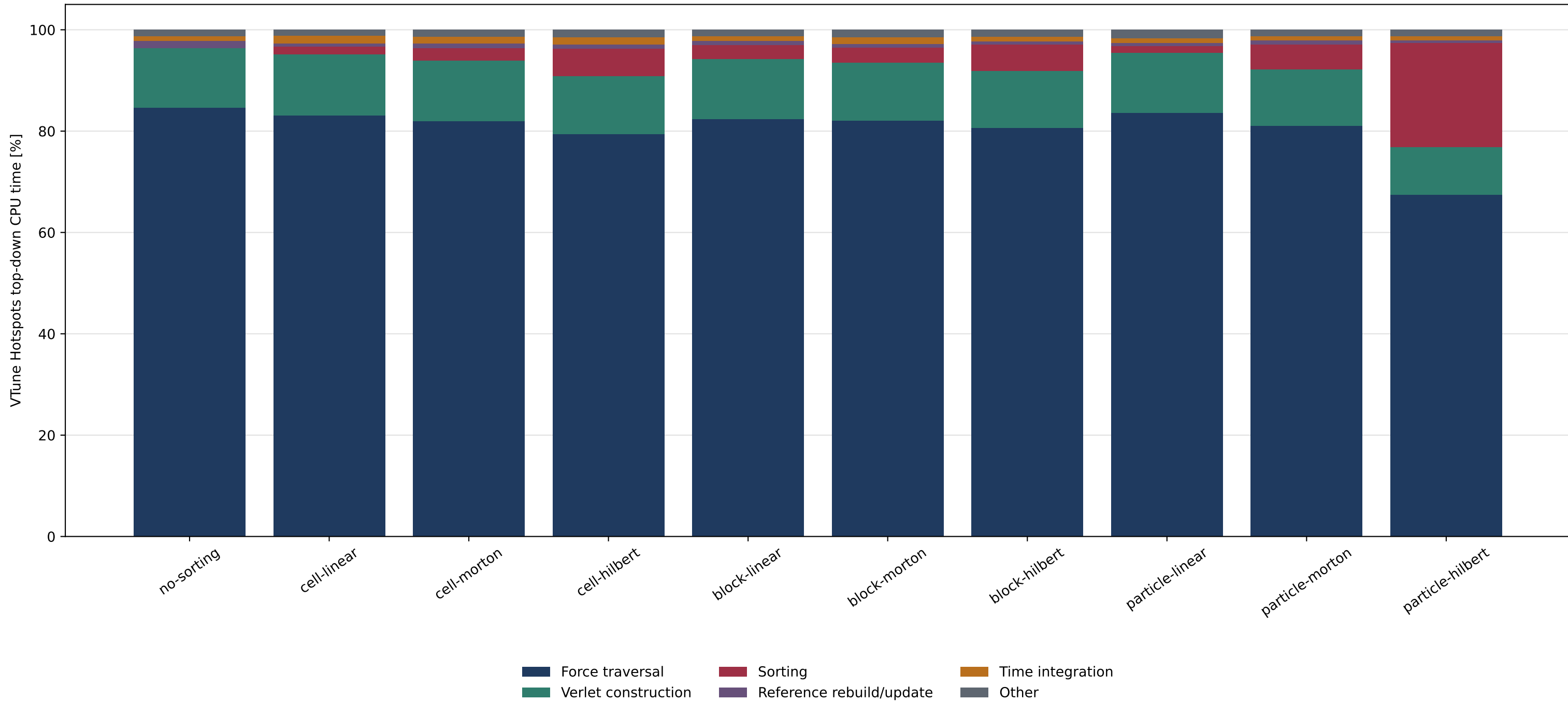
Runtime Decomposition by Phase
