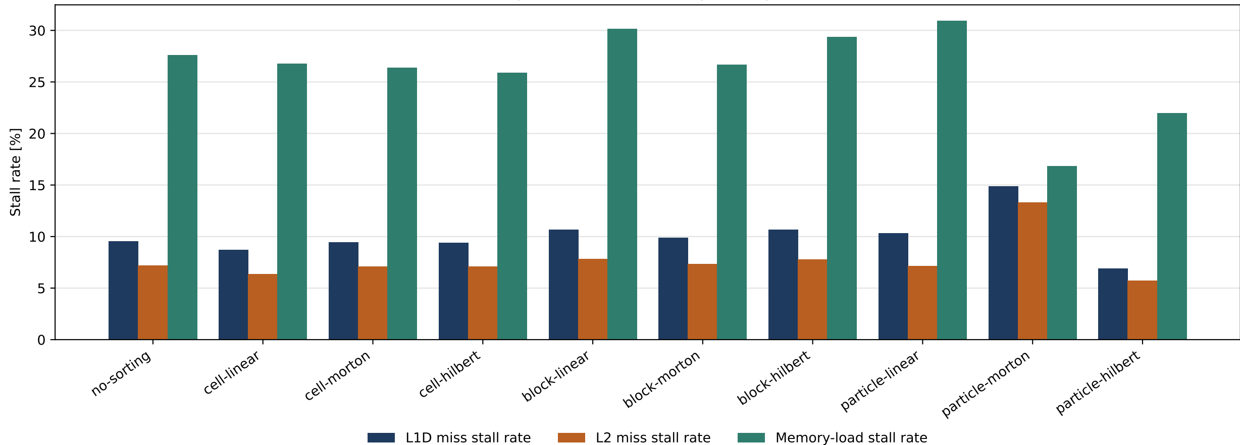
Memory-Related Stall Rates by Sorting Variant
