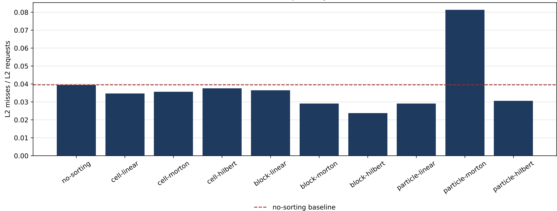
L2 Miss Ratio by Sorting Variant
