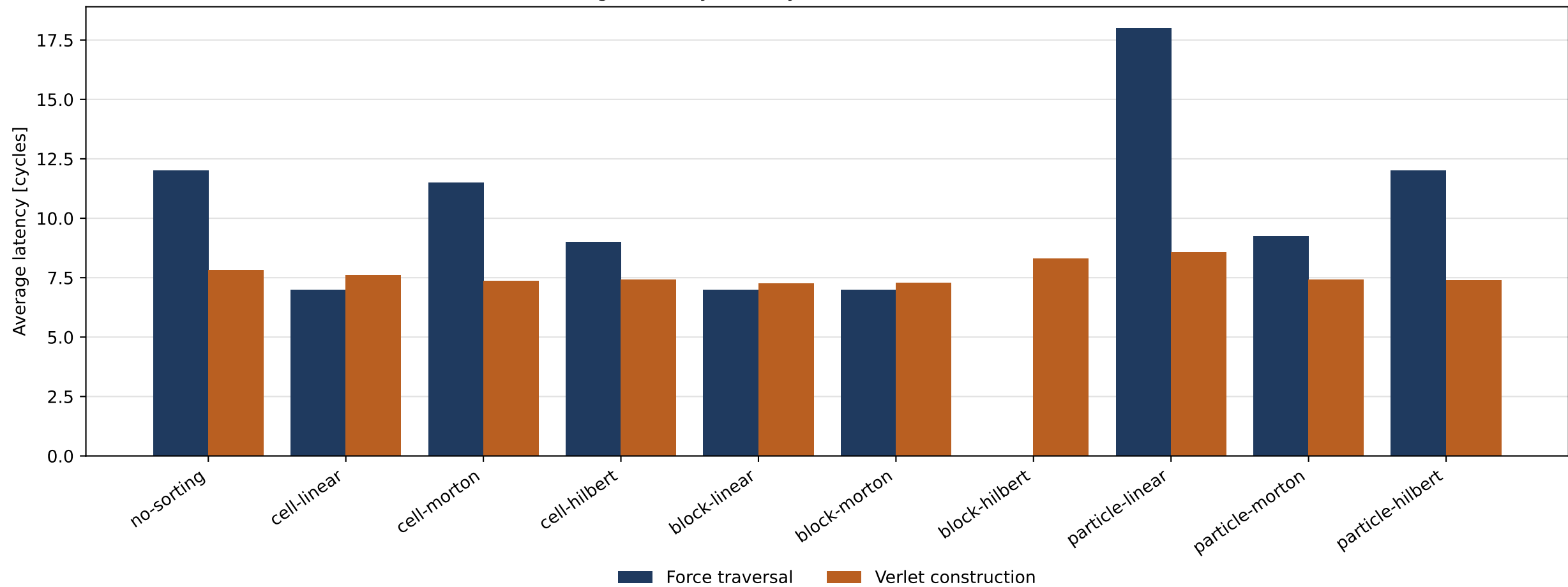
Average Memory Latency in Main Particle-Access Phases
