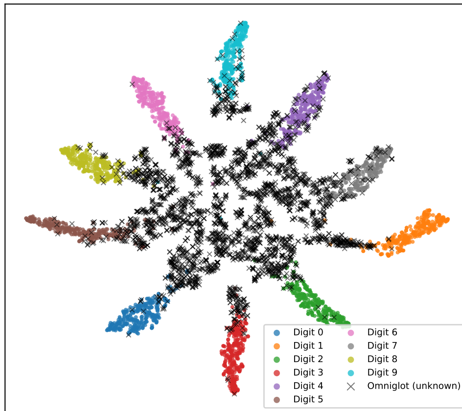
(b) MNIST / Omniglot - ResNet18
