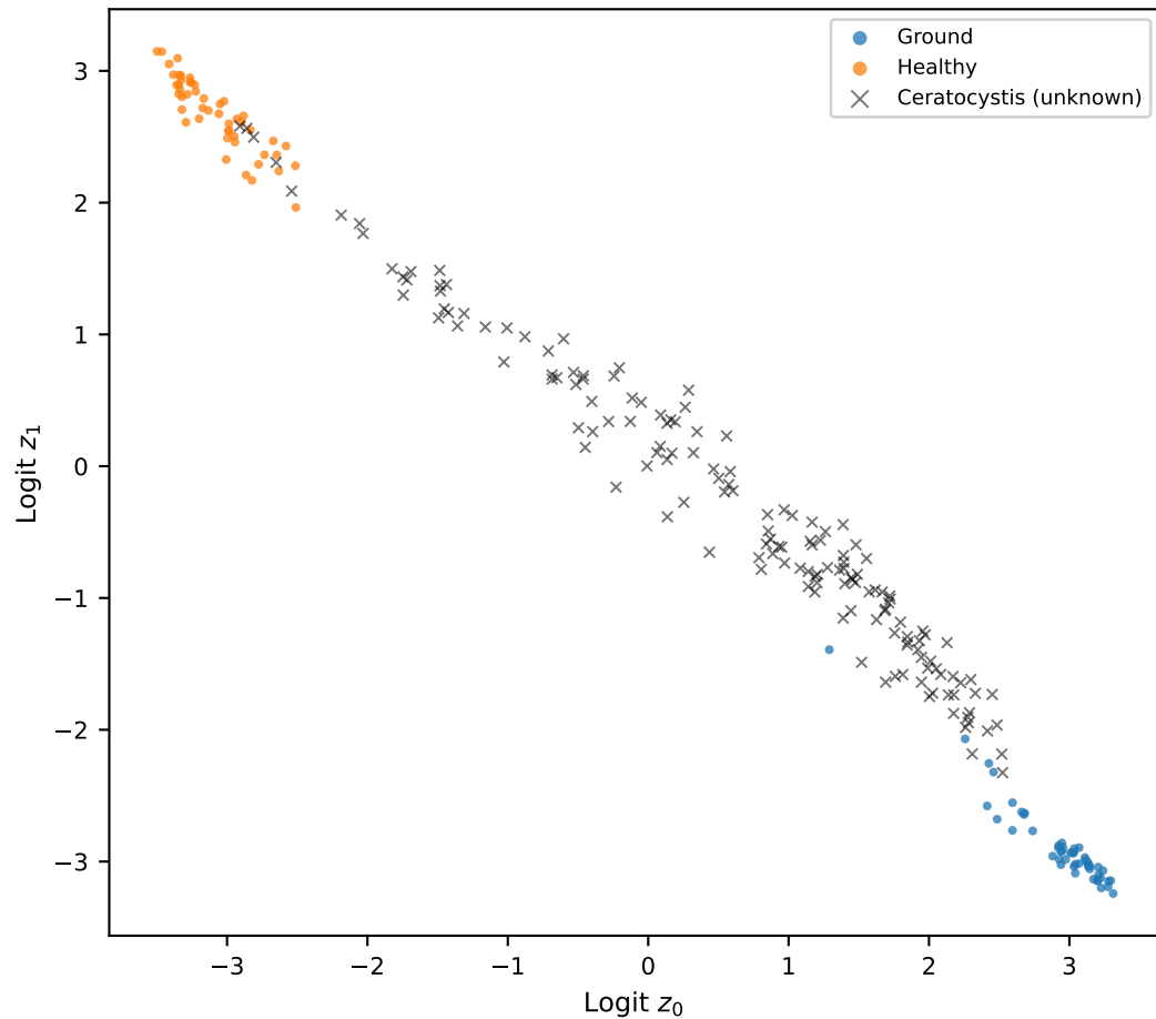
(a) Ceratocystis - AlexNet
