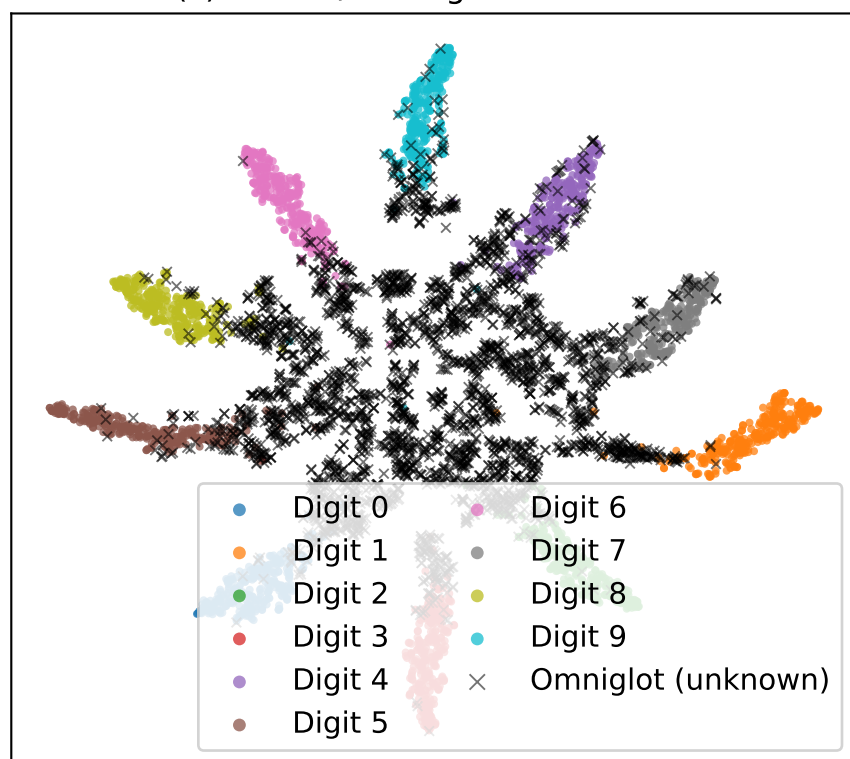
(c) MNIST / Omniglot - ResNet18
