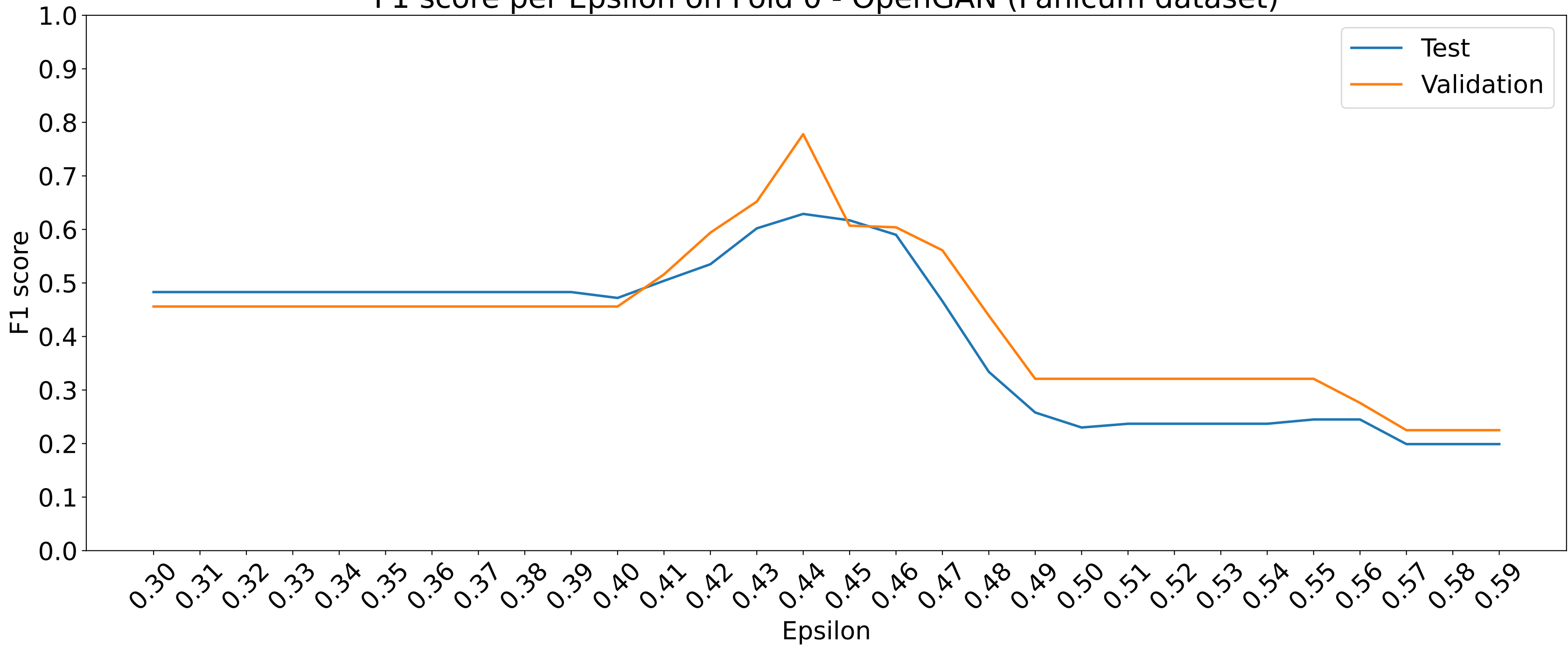
F1 score per Epsilon on Fold 0 - OpenGAN (Panicum dataset)
