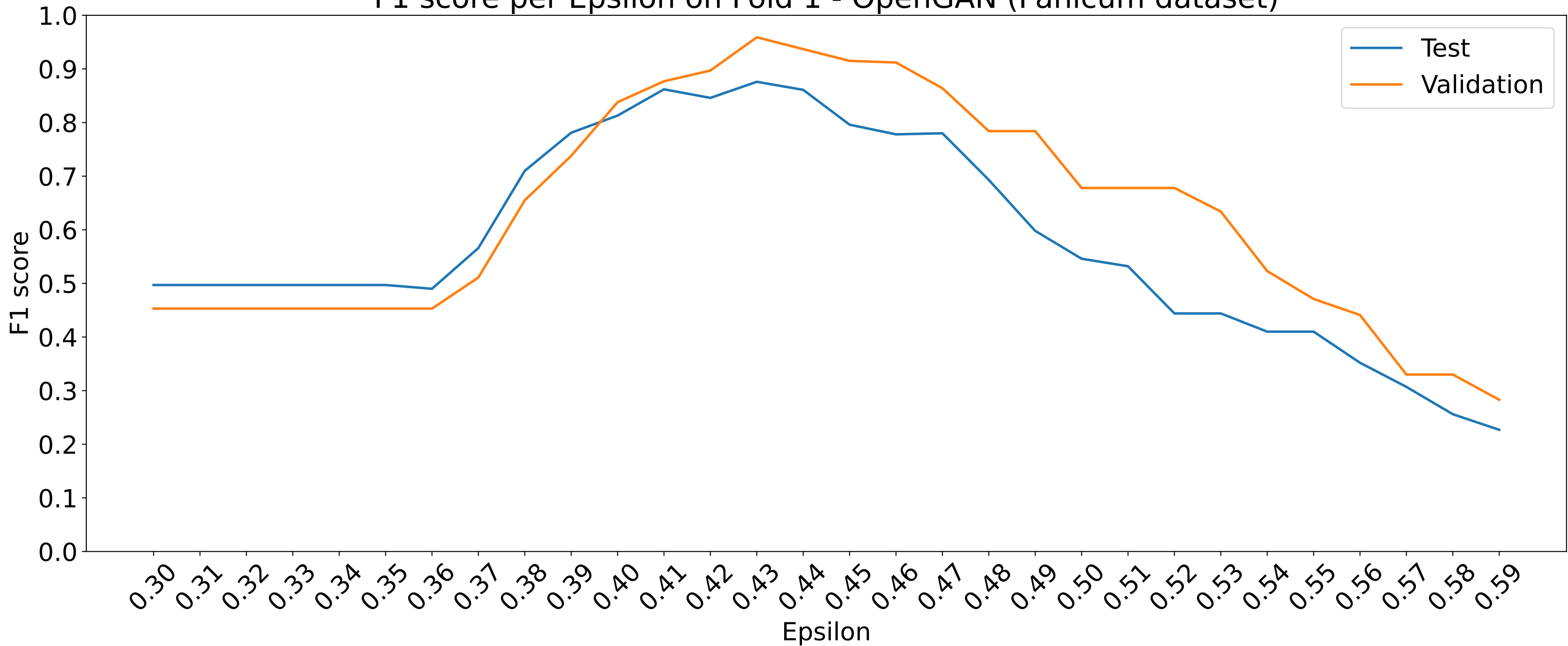
F1 score per Epsilon on Fold 1 - OpenGAN (Panicum dataset)
