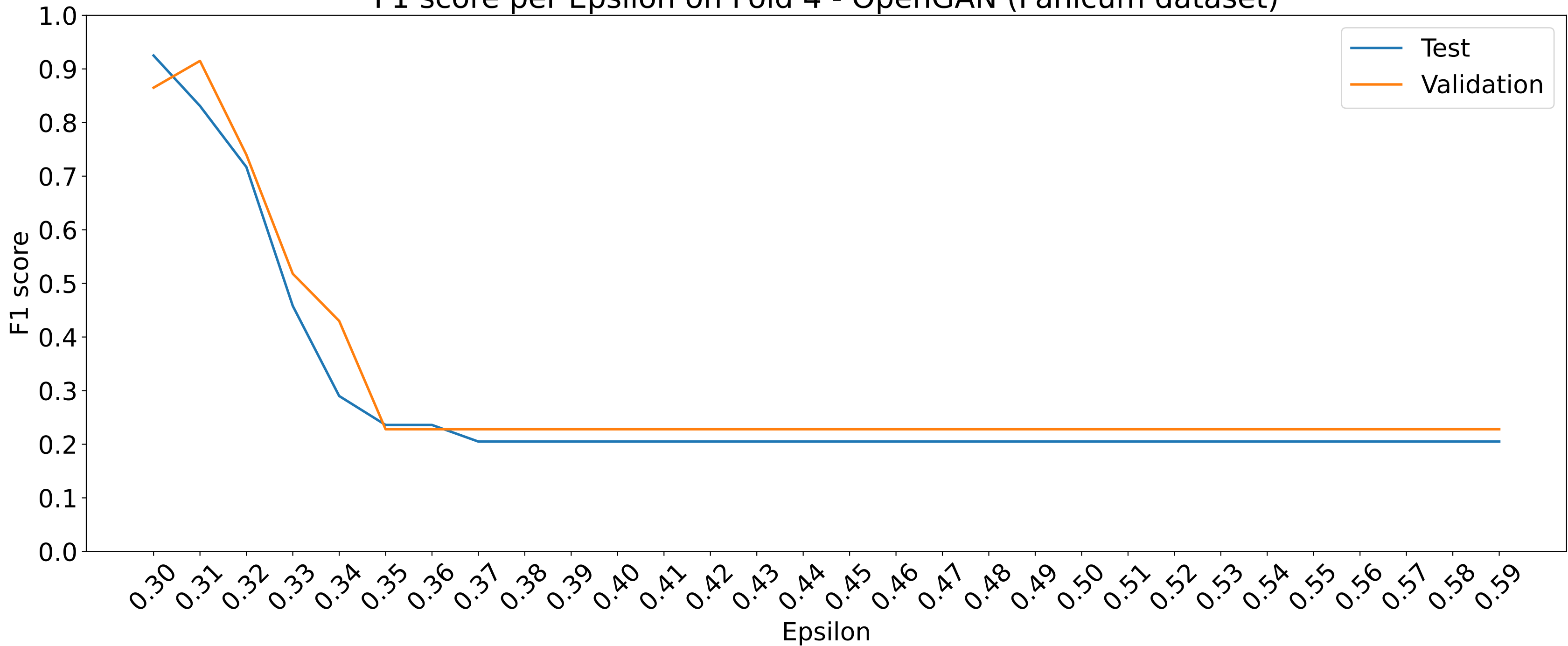
F1 score per Epsilon on Fold 4 - OpenGAN (Panicum dataset)
