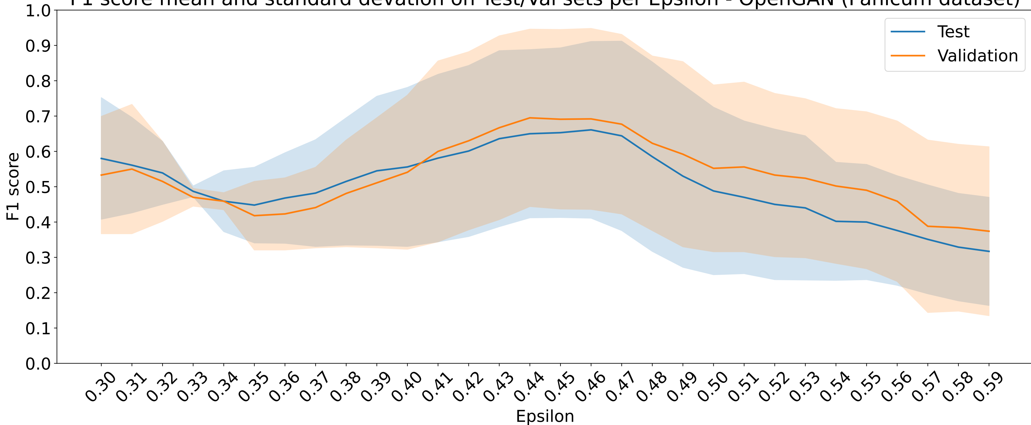
F1 score mean and standard deviation on Test/Val sets per Epsilon - OpenGAN (Panicum dataset)
