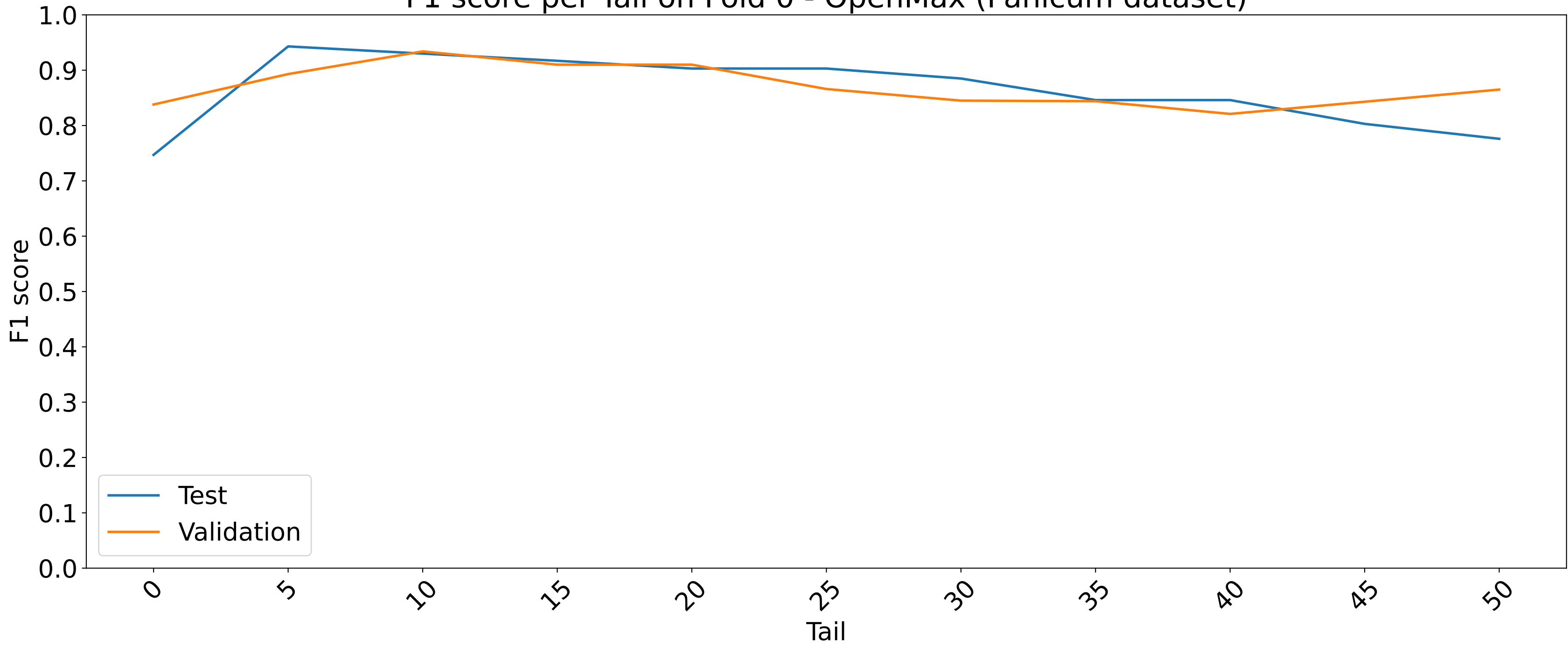
F1 score per Tail on Fold 0 - OpenMax (Panicum dataset)
