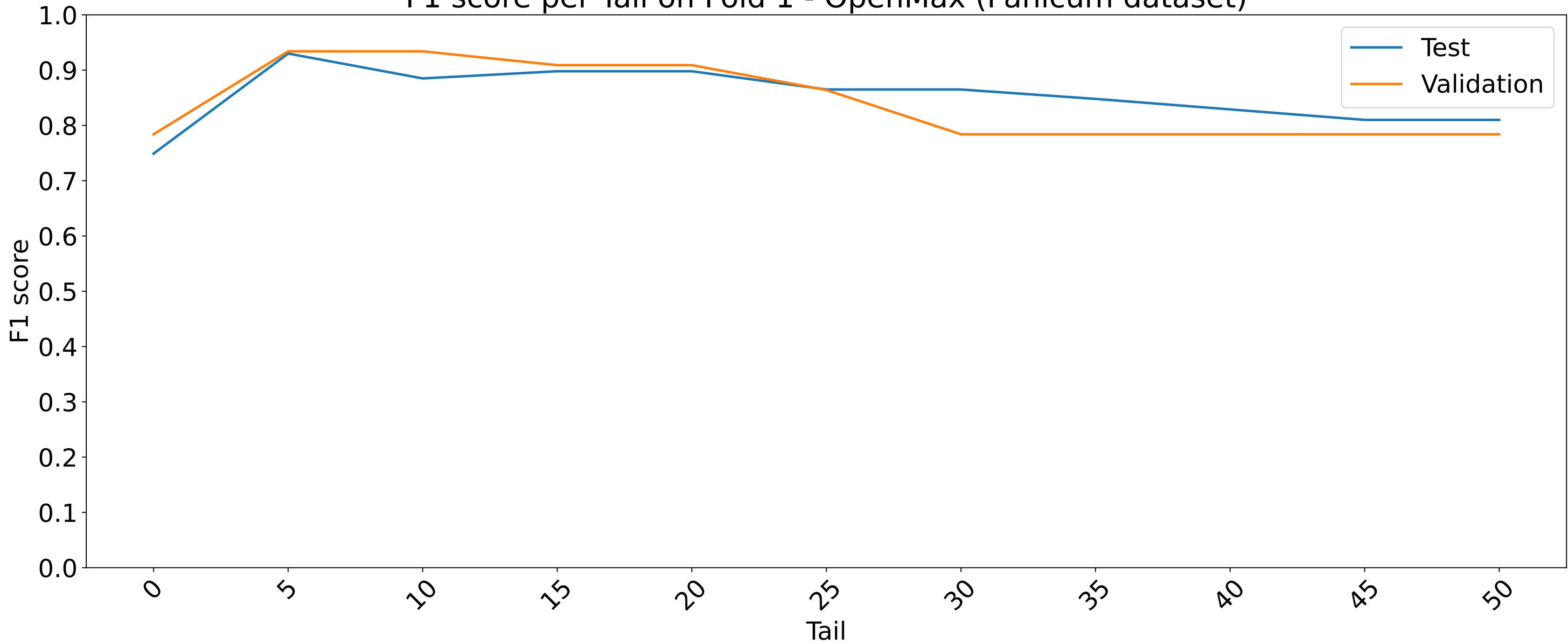
F1 score per Tail on Fold 1 - OpenMax (Panicum dataset)
