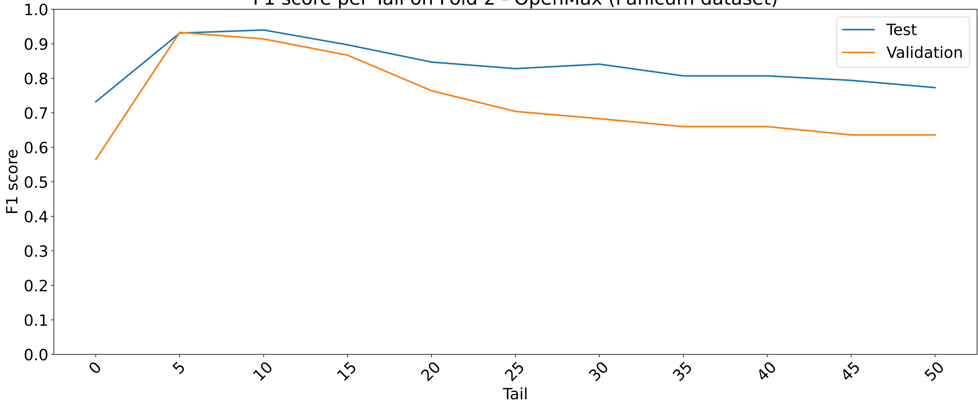
F1 score per Tail on Fold 2 - OpenMax (Panicum dataset)
