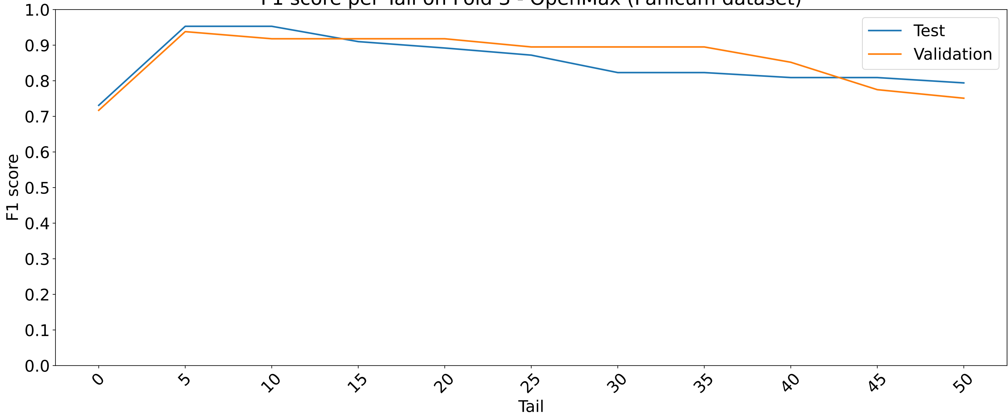
F1 score per Tail on Fold 3 - OpenMax (Panicum dataset)
