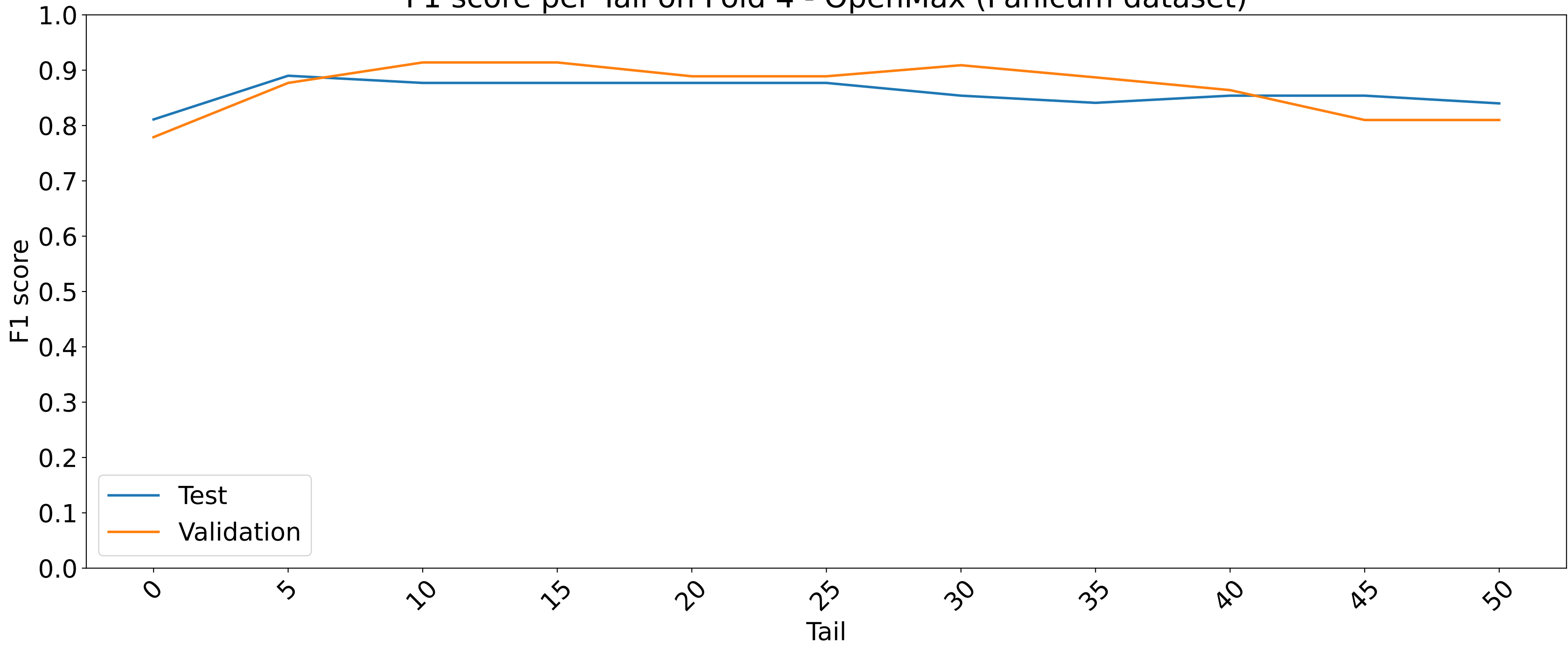
F1 score per Tail on Fold 4 - OpenMax (Panicum dataset)
