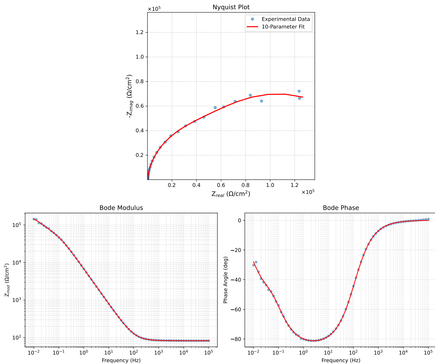
Figure 2: EIS Fit Results for Vasco_LN1_4_
