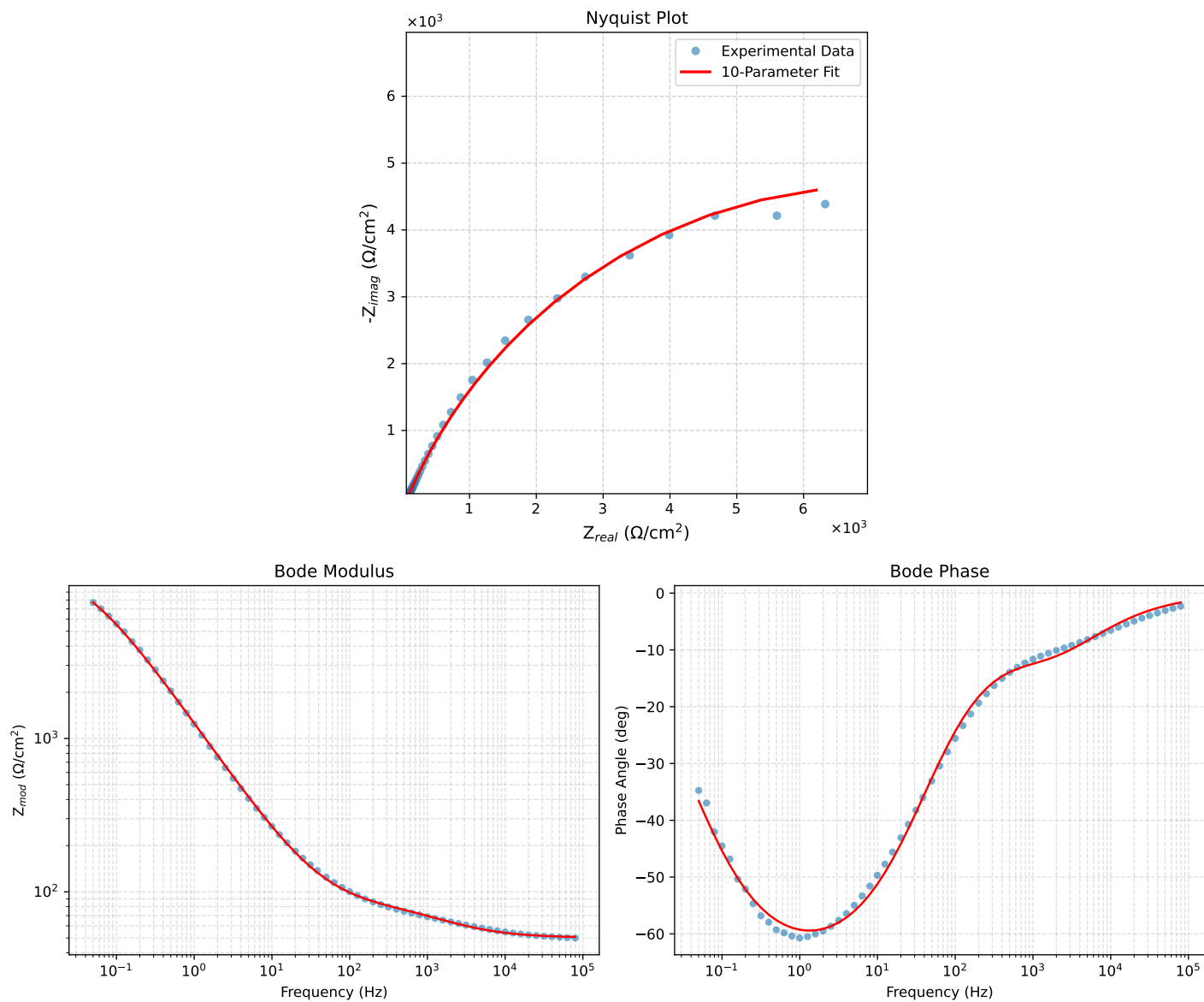
Figure 1: EIS Fit Results for Cauvel_5_NaVO3_1H
