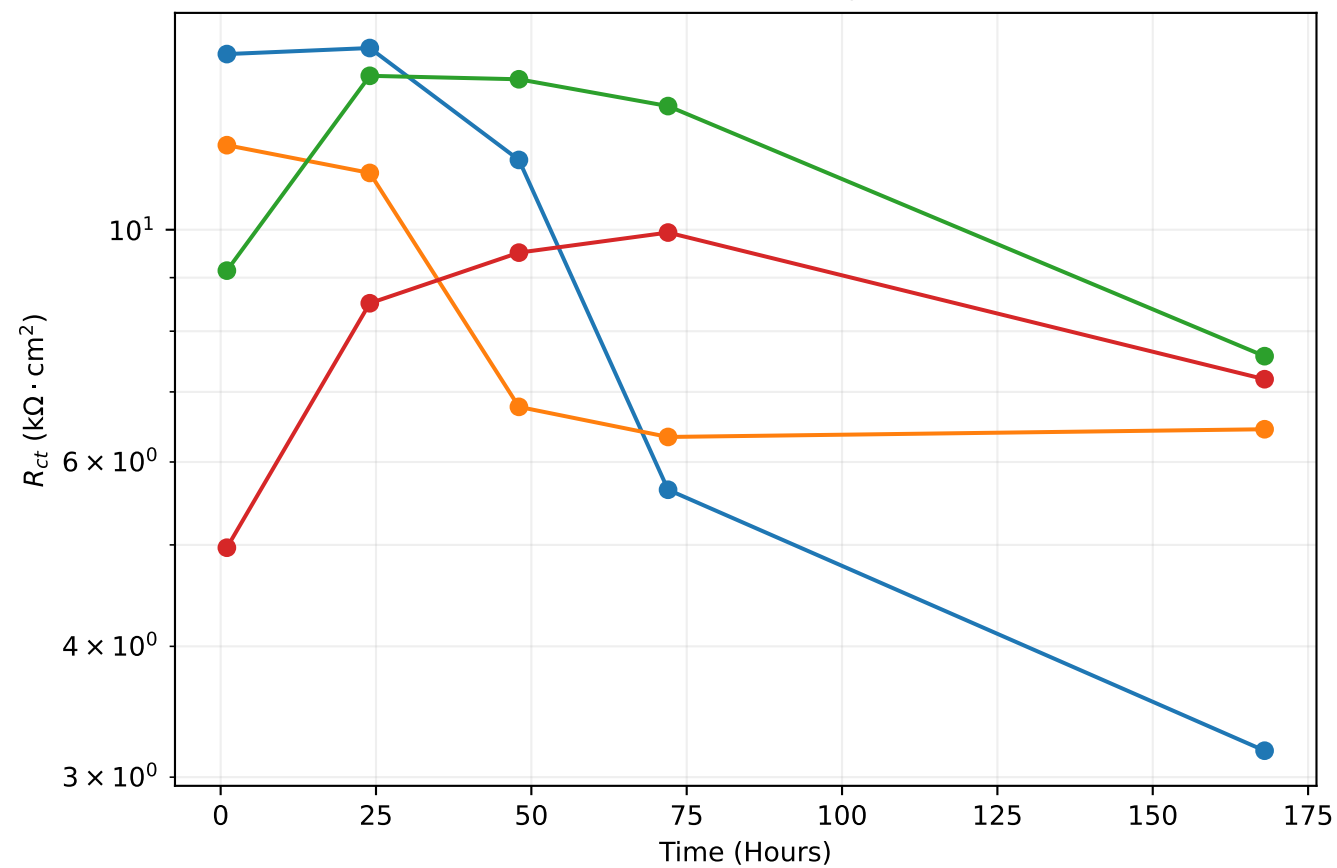
Evolution of R_{ct}
