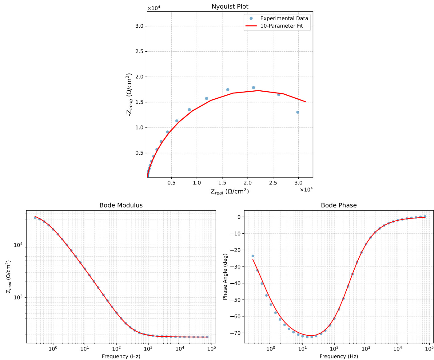
Figure 1: EIS Fit Results for CZn-2control_0.05MCl_1
