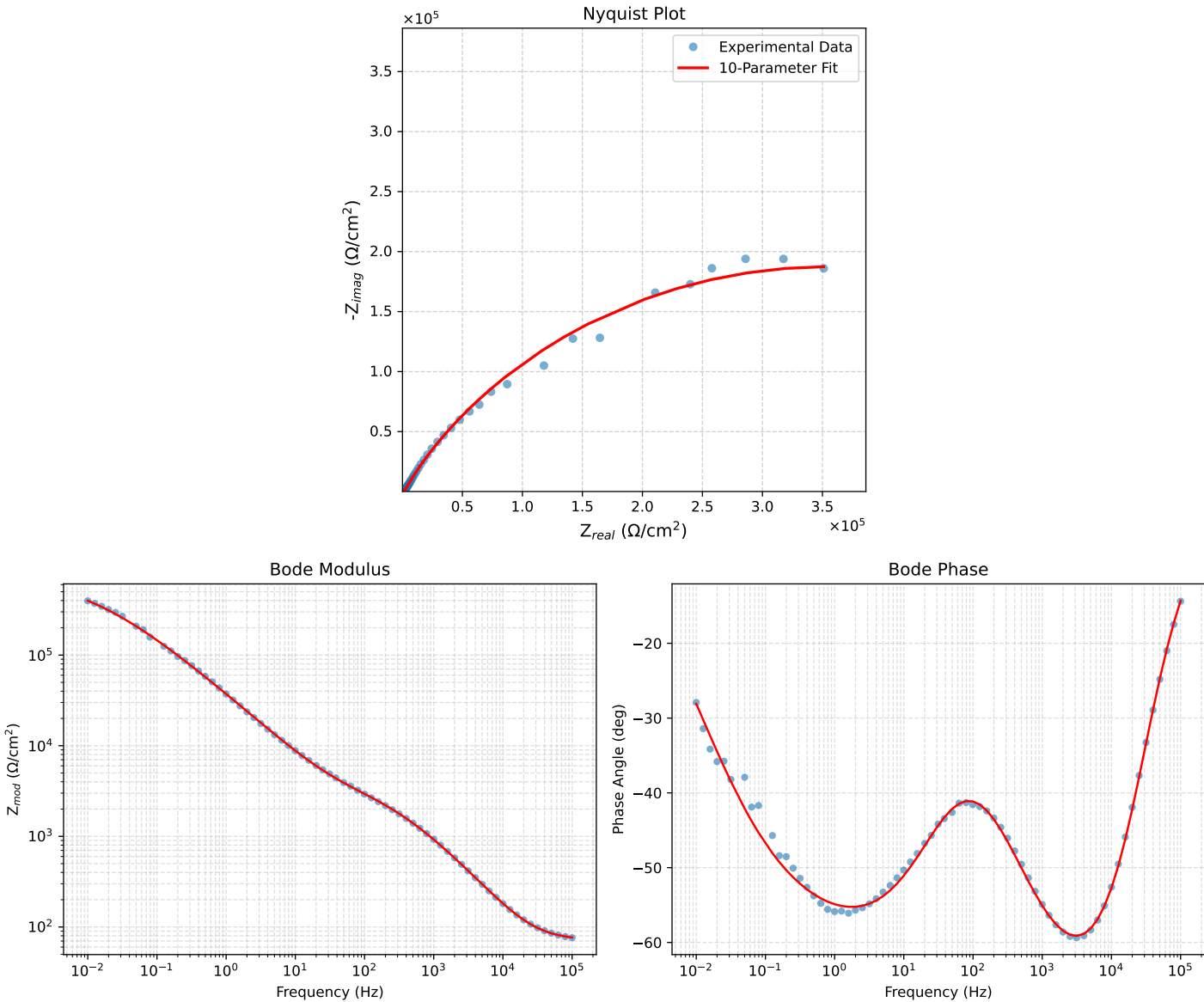
Figure 4: EIS Fit Results for PNA_1.1.7d-1 - Copy
