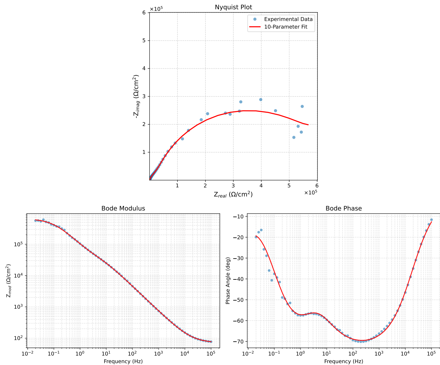
Figure 2: EIS Fit Results for PNA_1_1_1h
