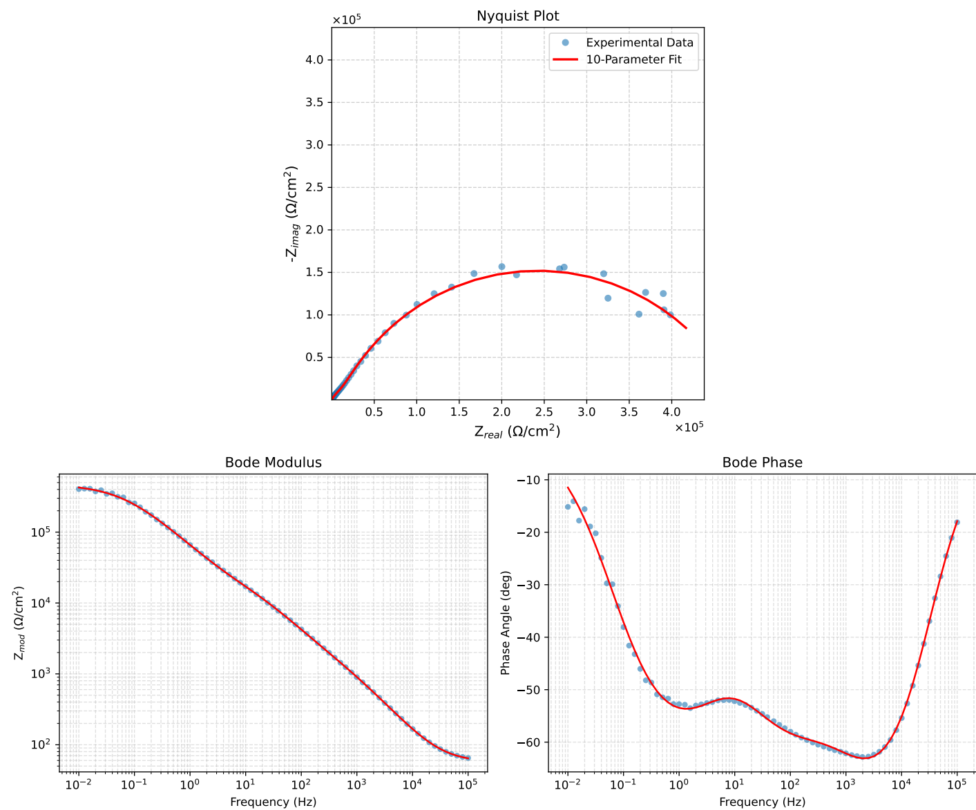
Figure 1: EIS Fit Results for PNA_1_1_1d
