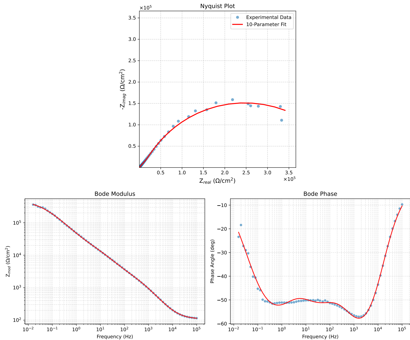
Figure 3: EIS Fit Results for PNA_1.1.3d - Copy
