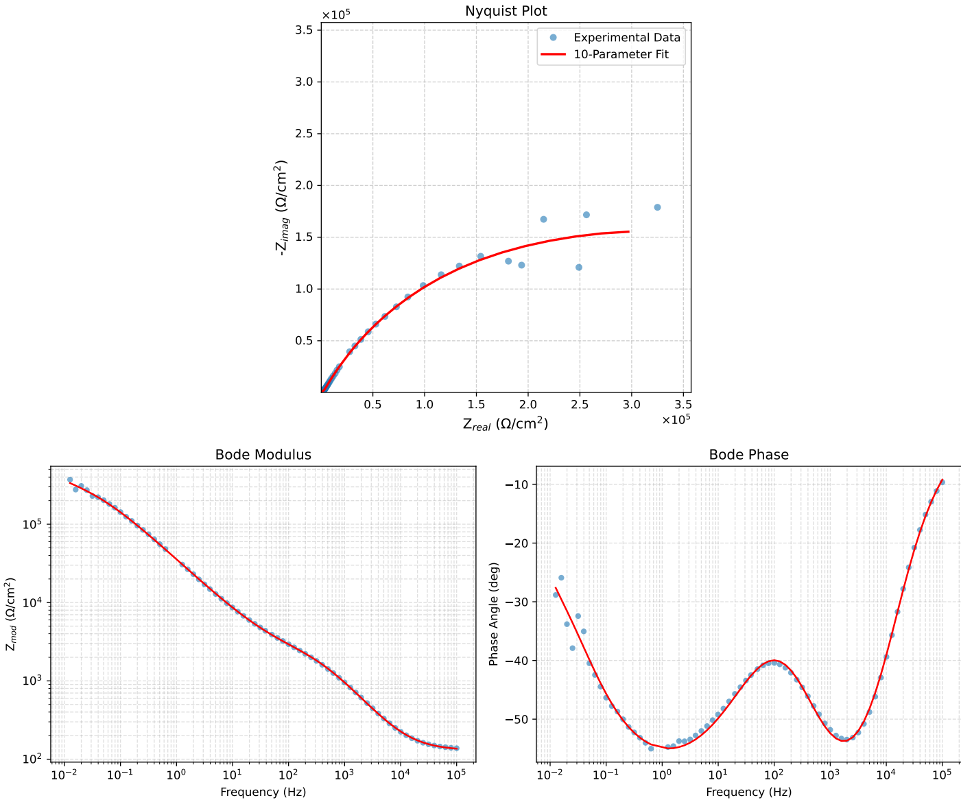
Figure 5: EIS Fit Results for PNA_1.1_7d-2 - Copy
