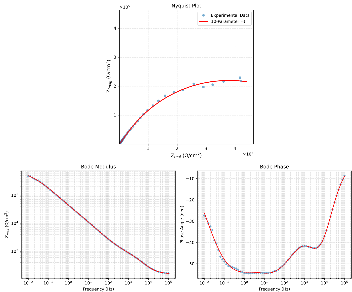
Figure 4: EIS Fit Results for PNA_2_2_3d
