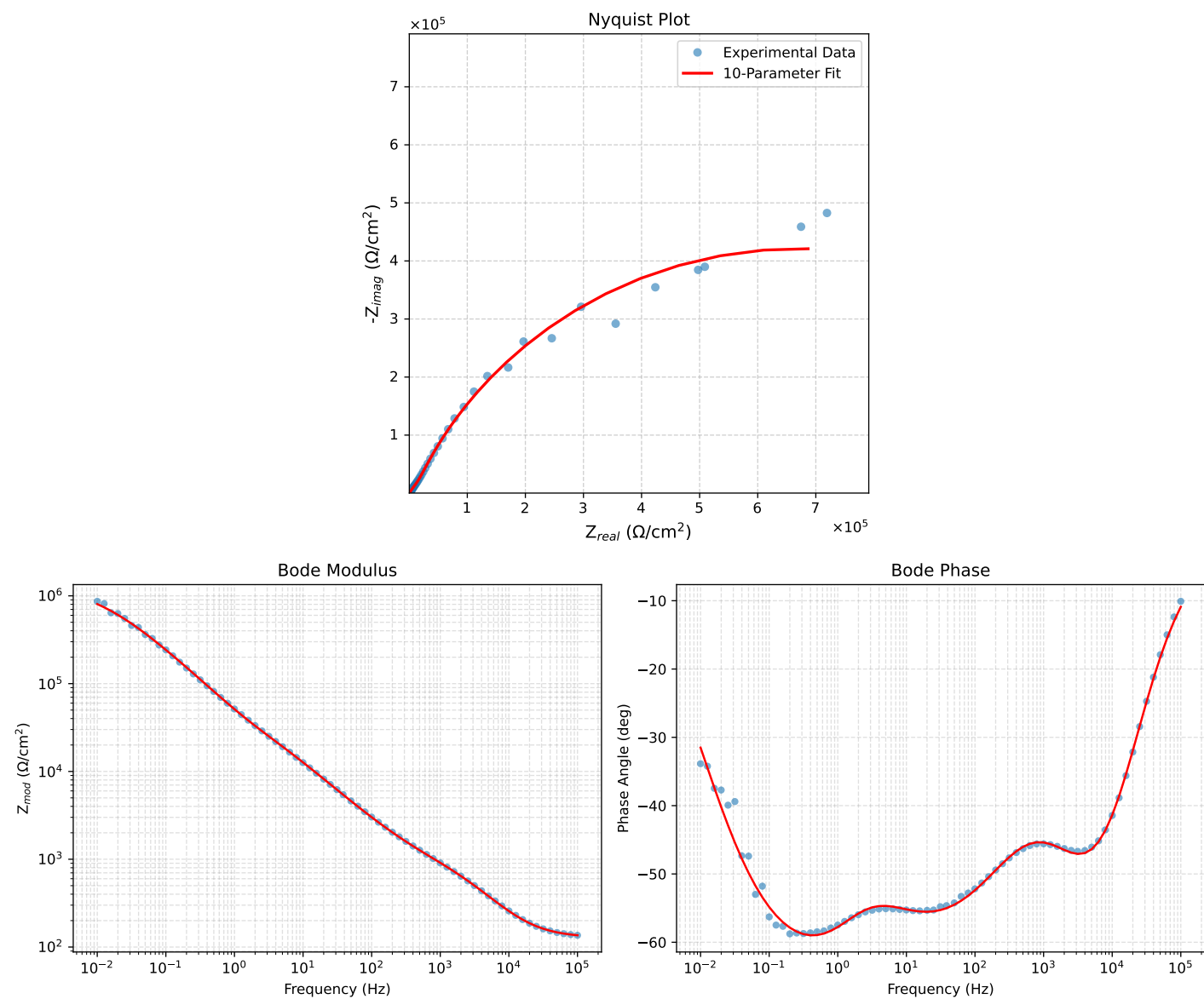
Figure 2: EIS Fit Results for PNA_2.2.1d
