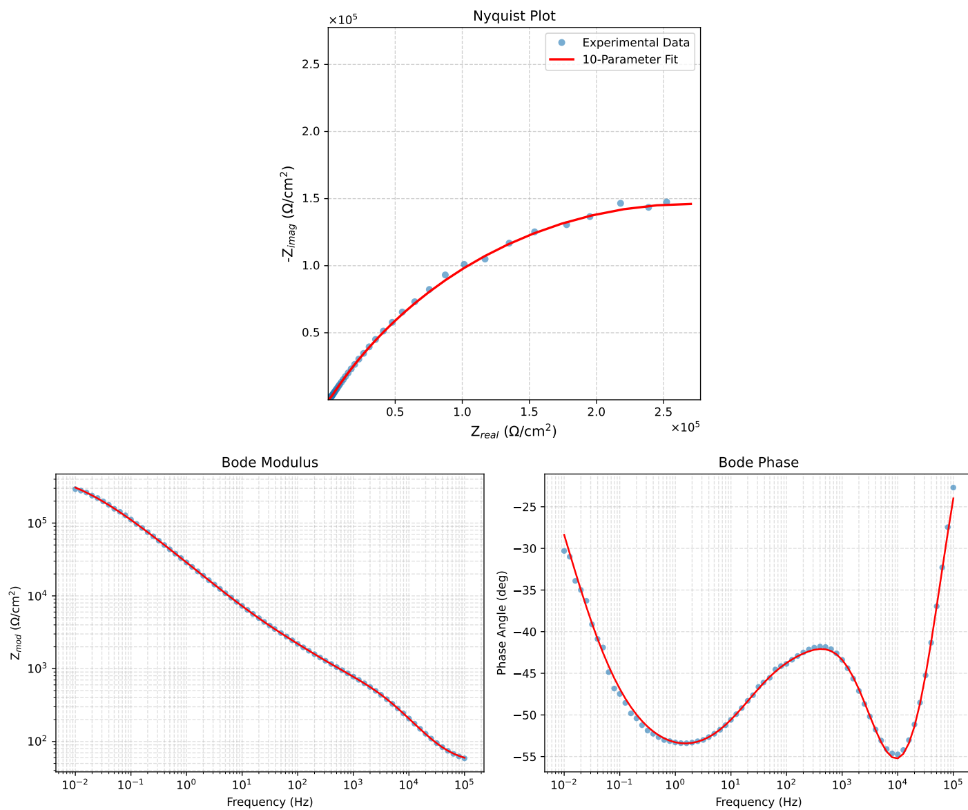
Figure 5: EIS Fit Results for PNA_2_2_7d
