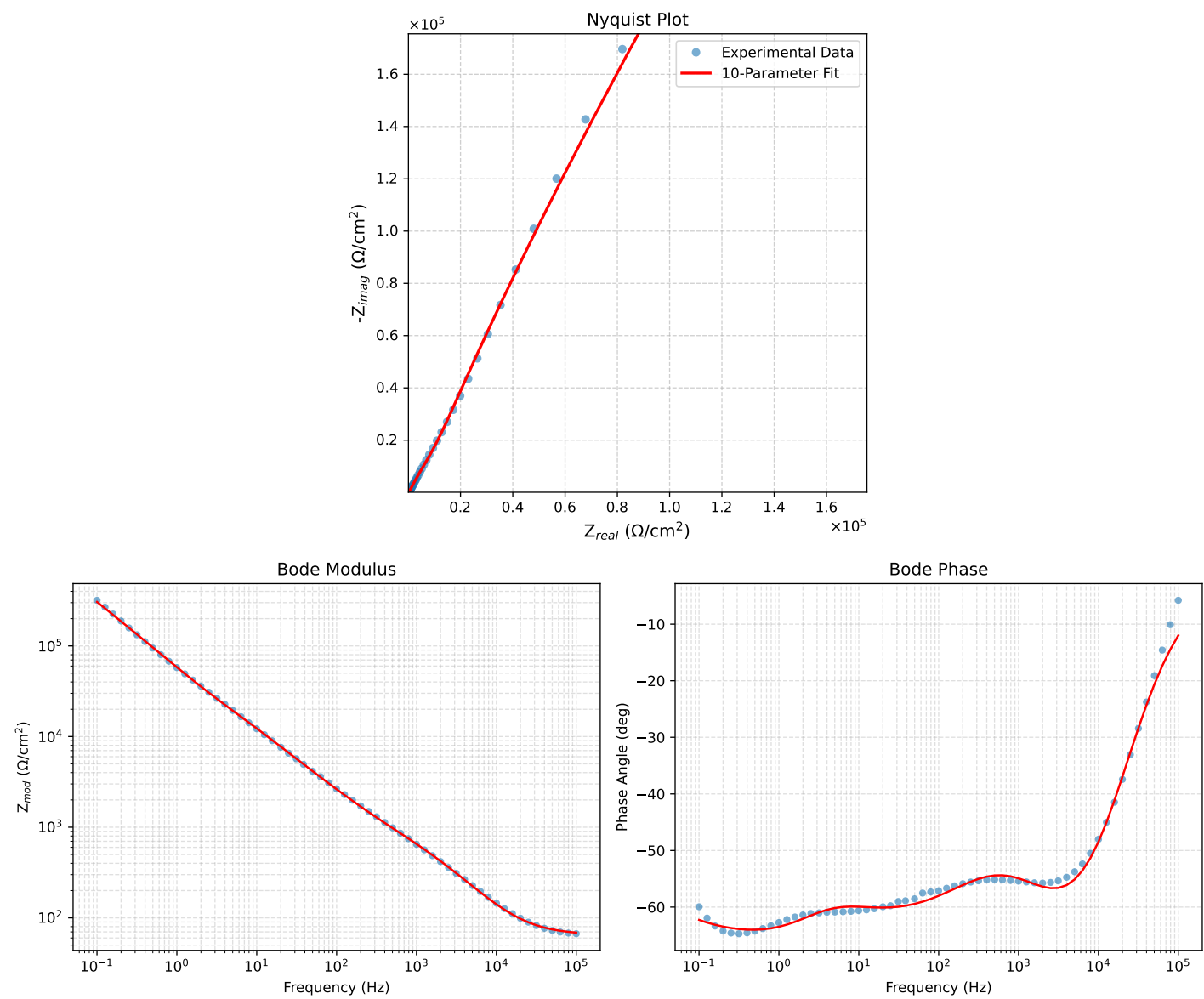
Figure 1: EIS Fit Results for PNA_2.2_0h-1
