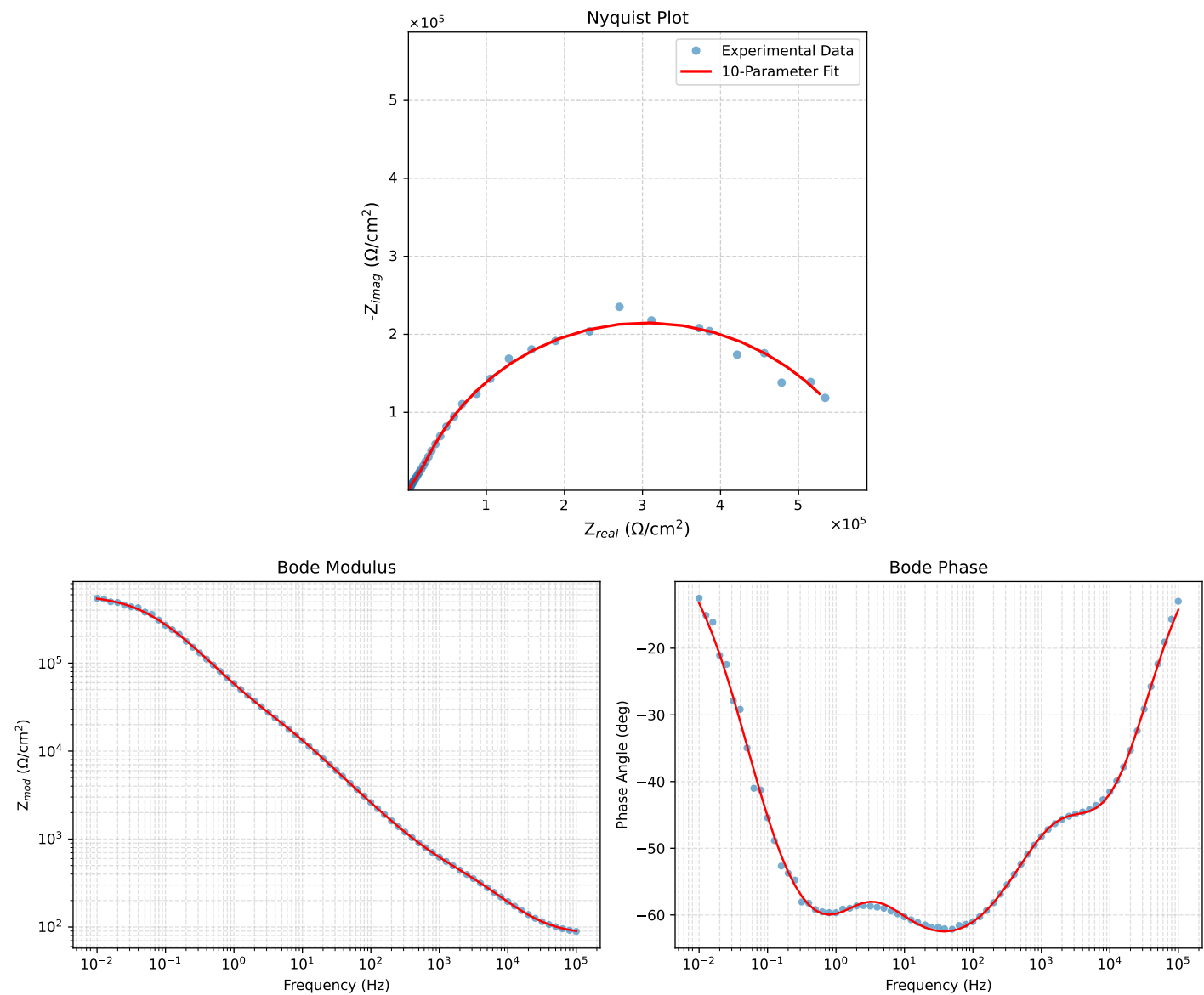
Figure 3: EIS Fit Results for PNA_2.2.1h
