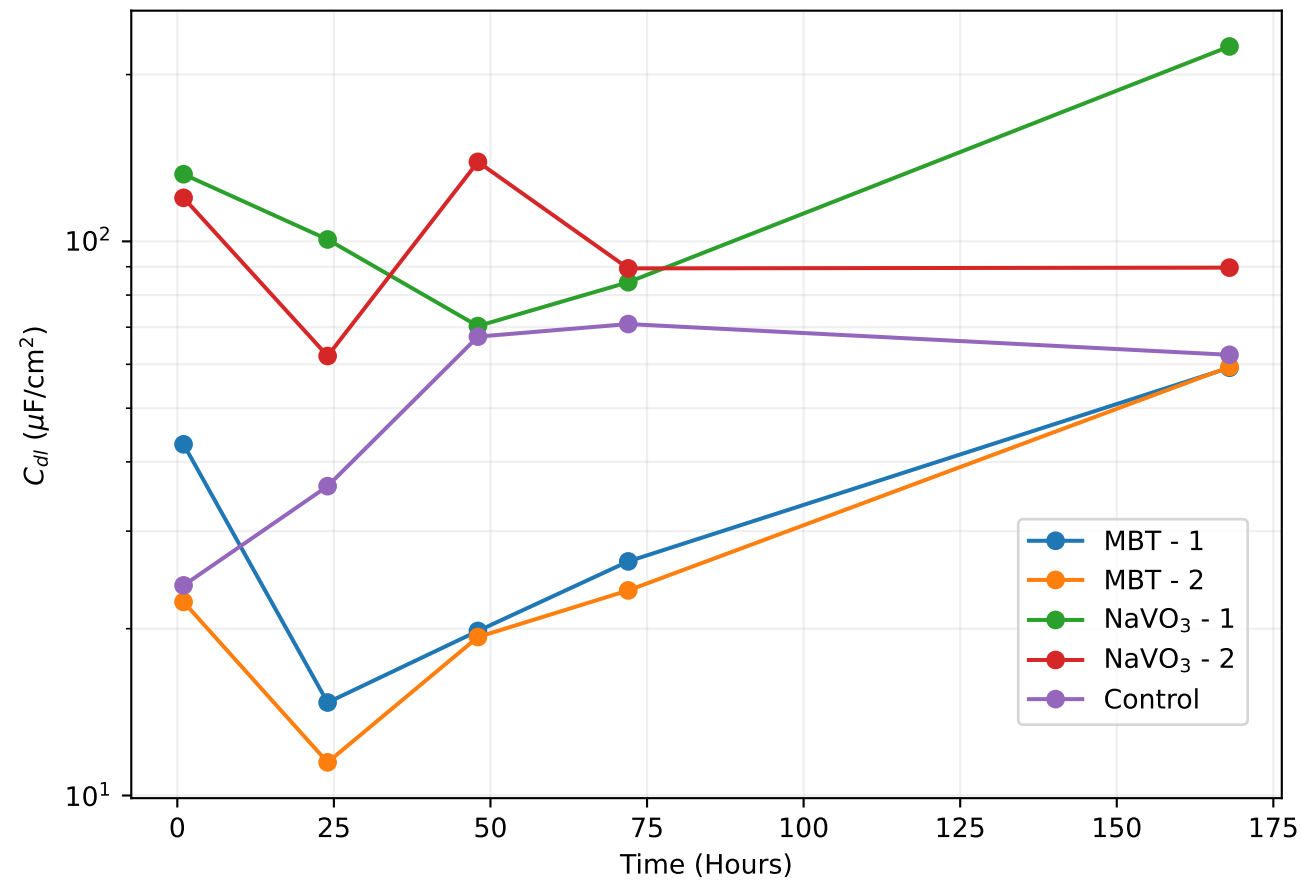
Evolution of C_{dl}
