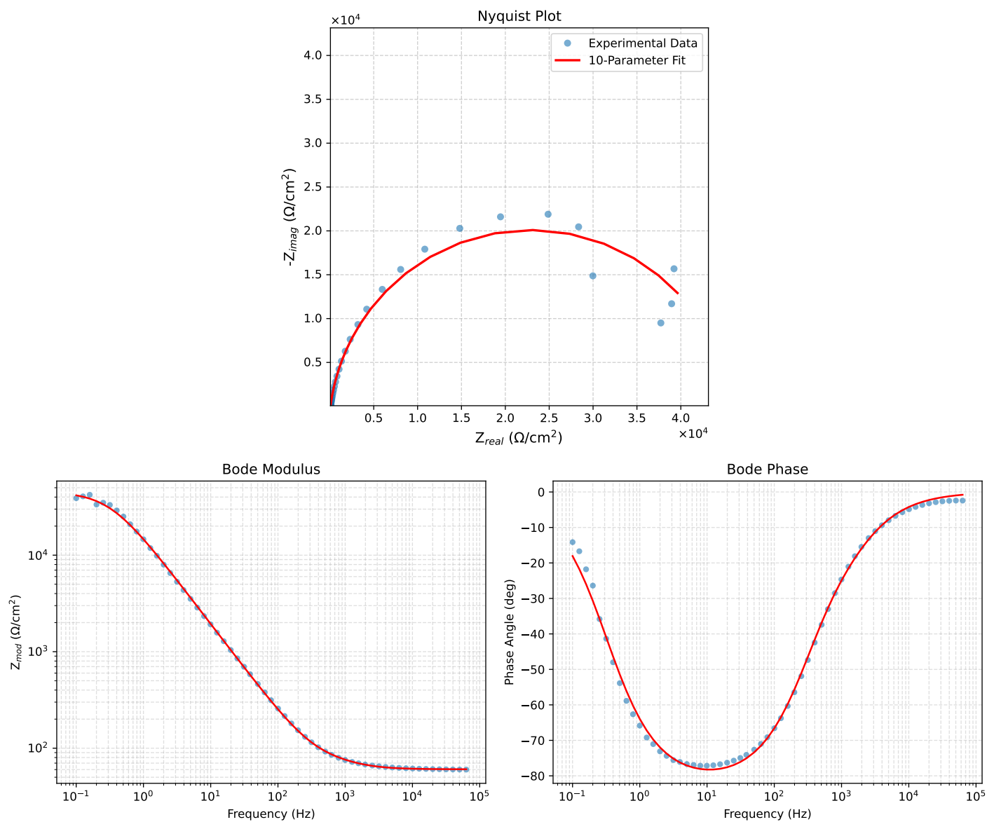
Figure 1: EIS Fit Results for Cauvel_2.8HQ_1H
