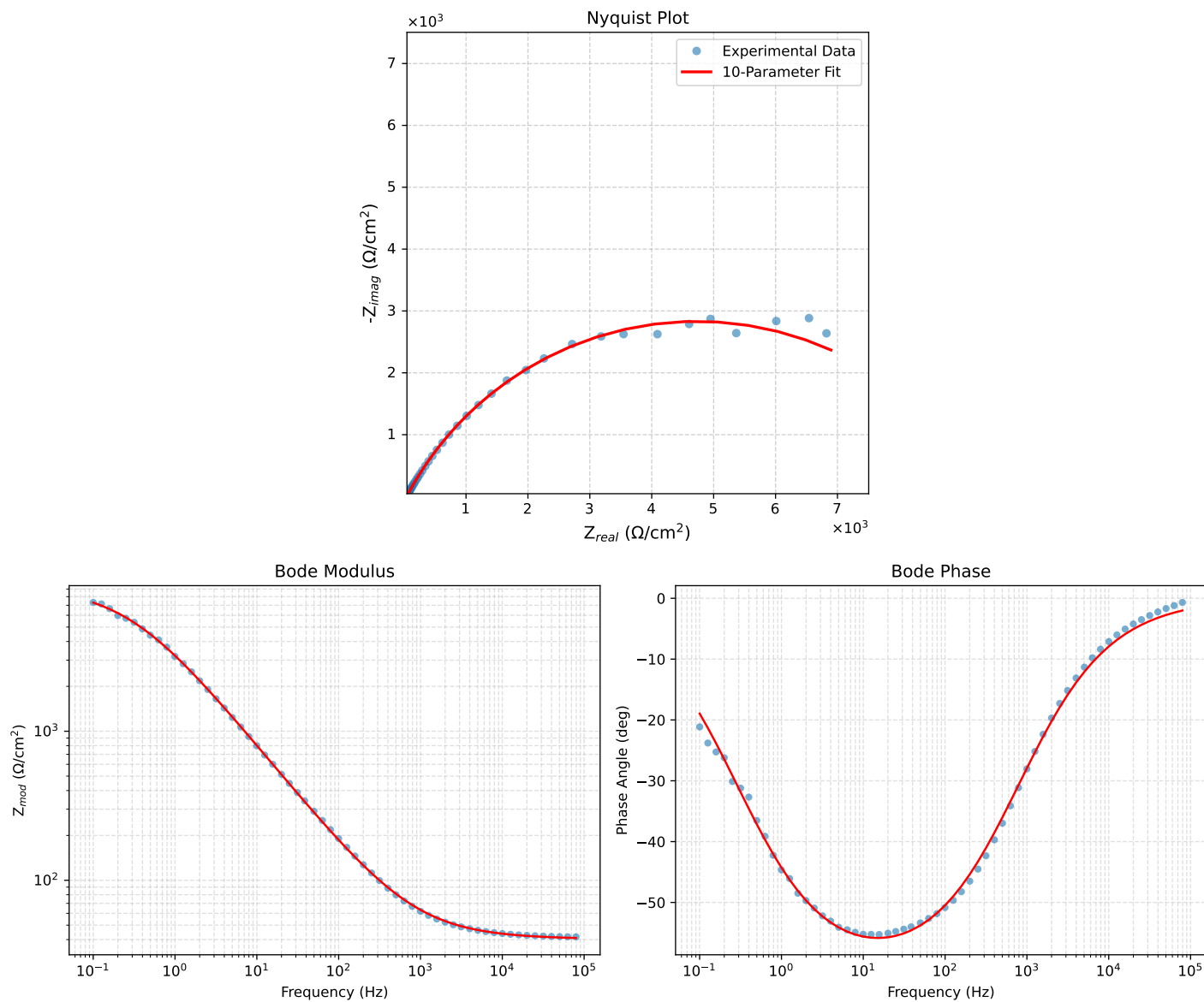
Figure 1: EIS Fit Results for Cauvel_II_NaVO3.1H
