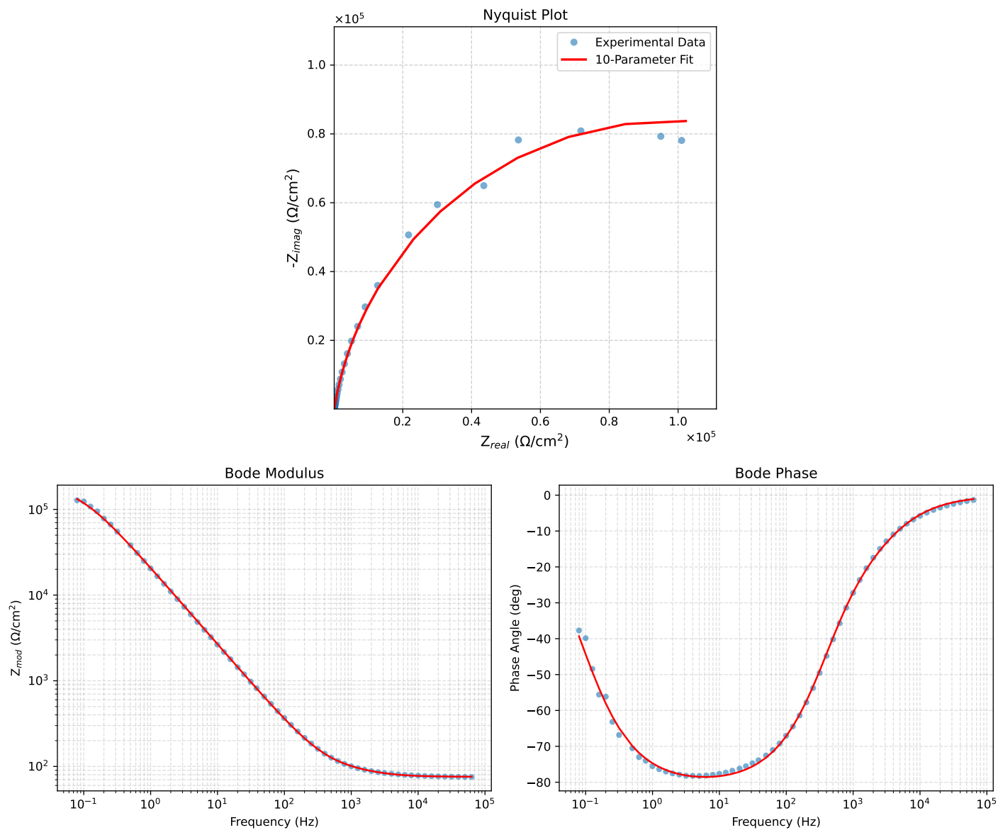
Figure 1: EIS Fit Results for Cauvel.1_Lcystine_4H
