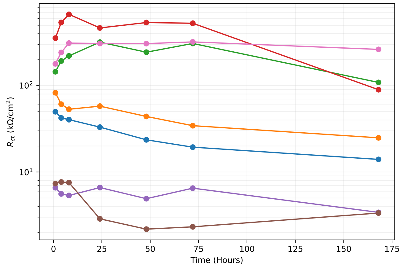
Evolution of R_{ct}
