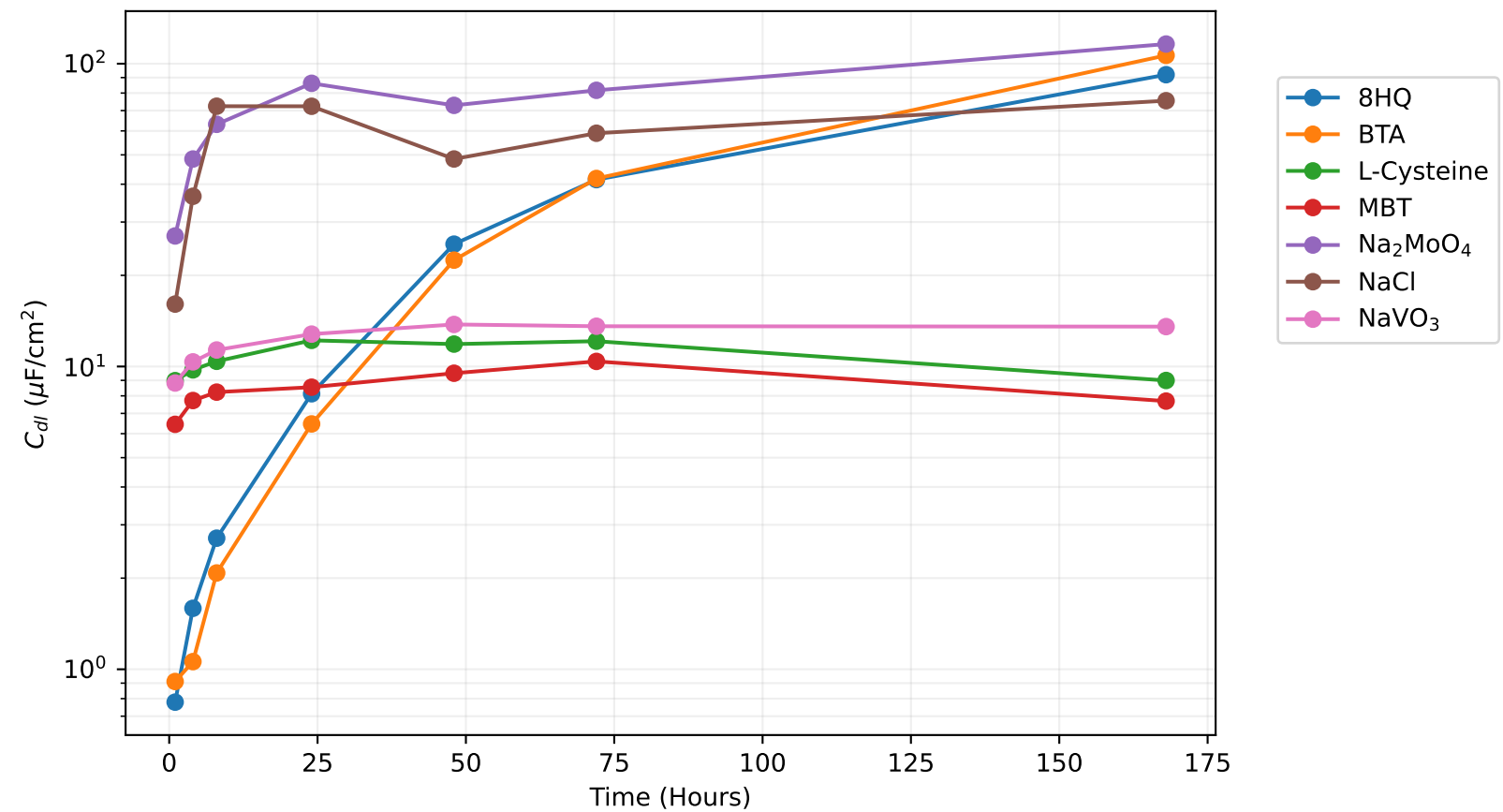
Evolution of C_{dl}
