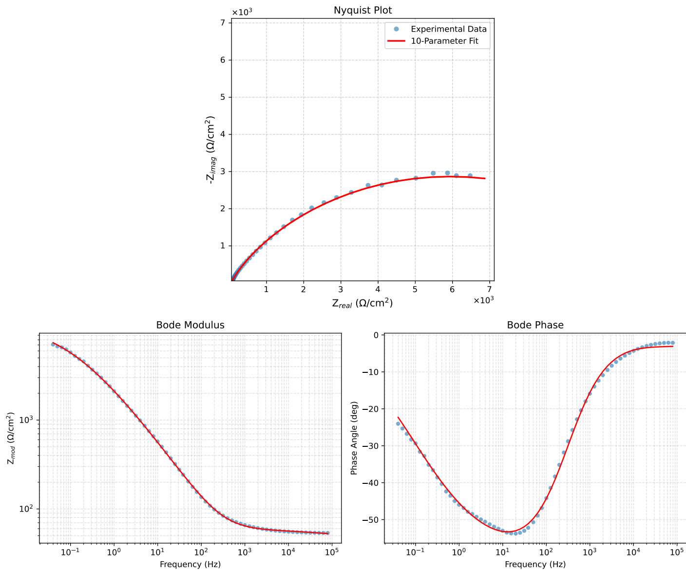
Figure 1: EIS Fit Results for Cauvel_IL-NaVO3-24H
