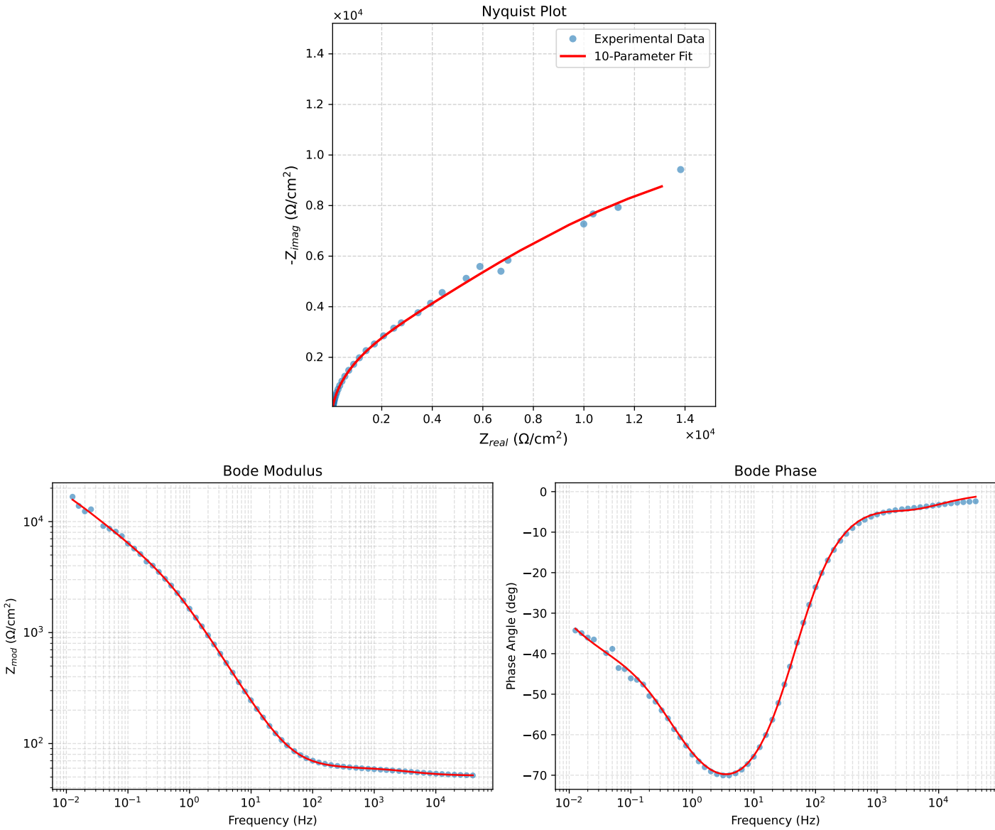
Figure 1: EIS Fit Results for Cauvel_3_Mo_48H
