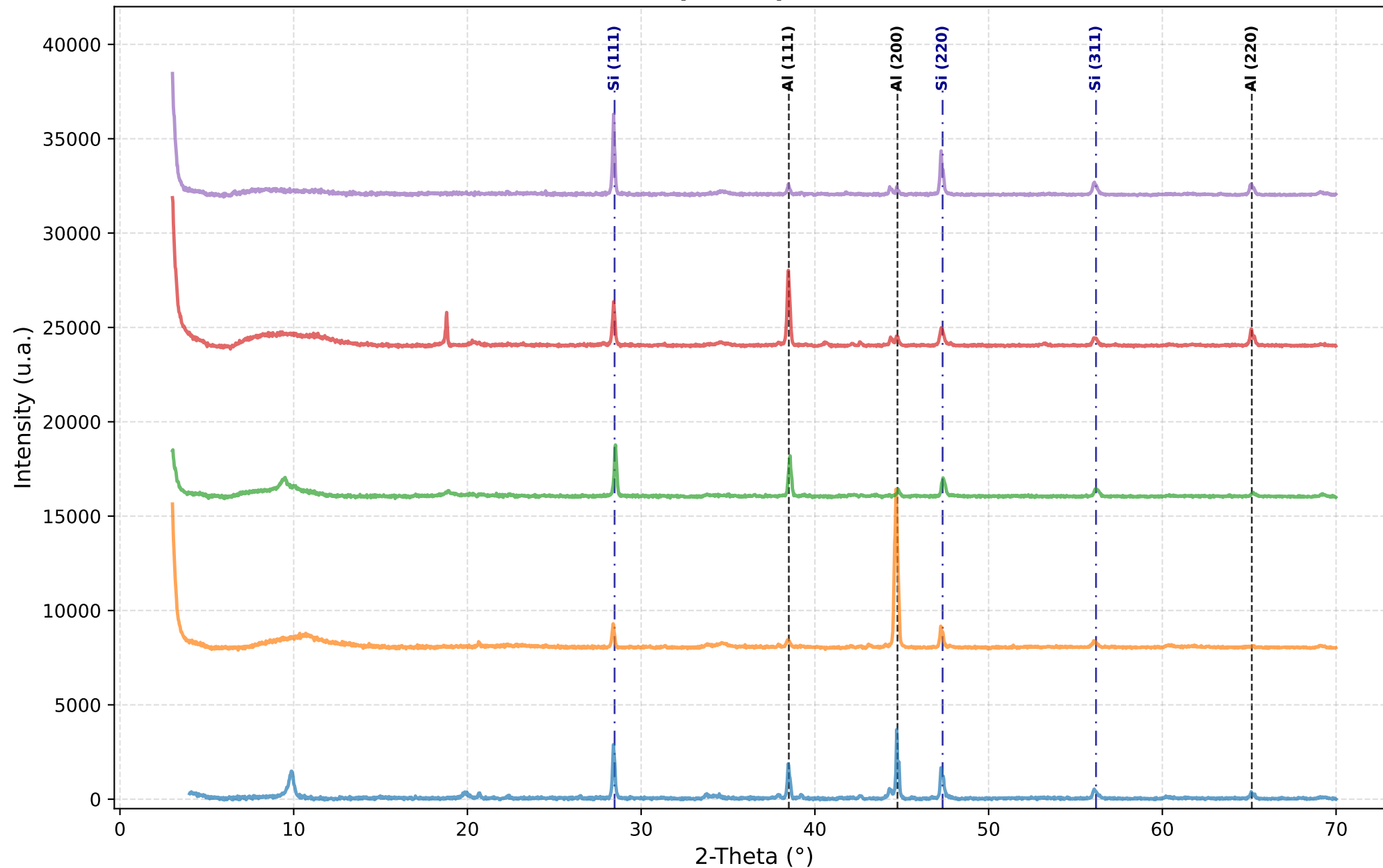
Complete Spectrum
