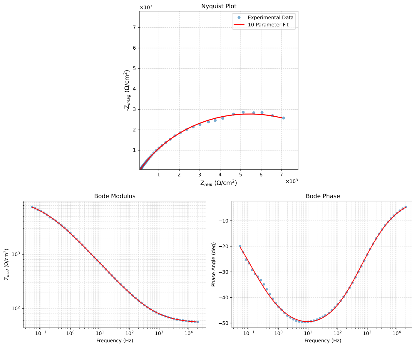
Figure 1: EIS Fit Results for Cauvel_7_NaVO3_1H
