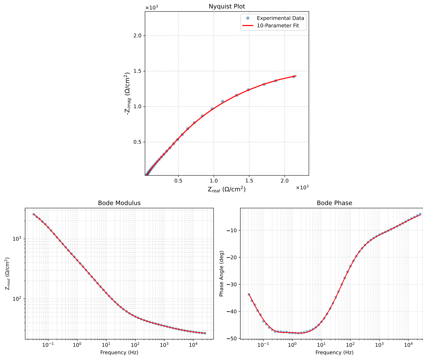
Figure 1: EIS Fit Results for CaueI_III_NaVO3-168H
