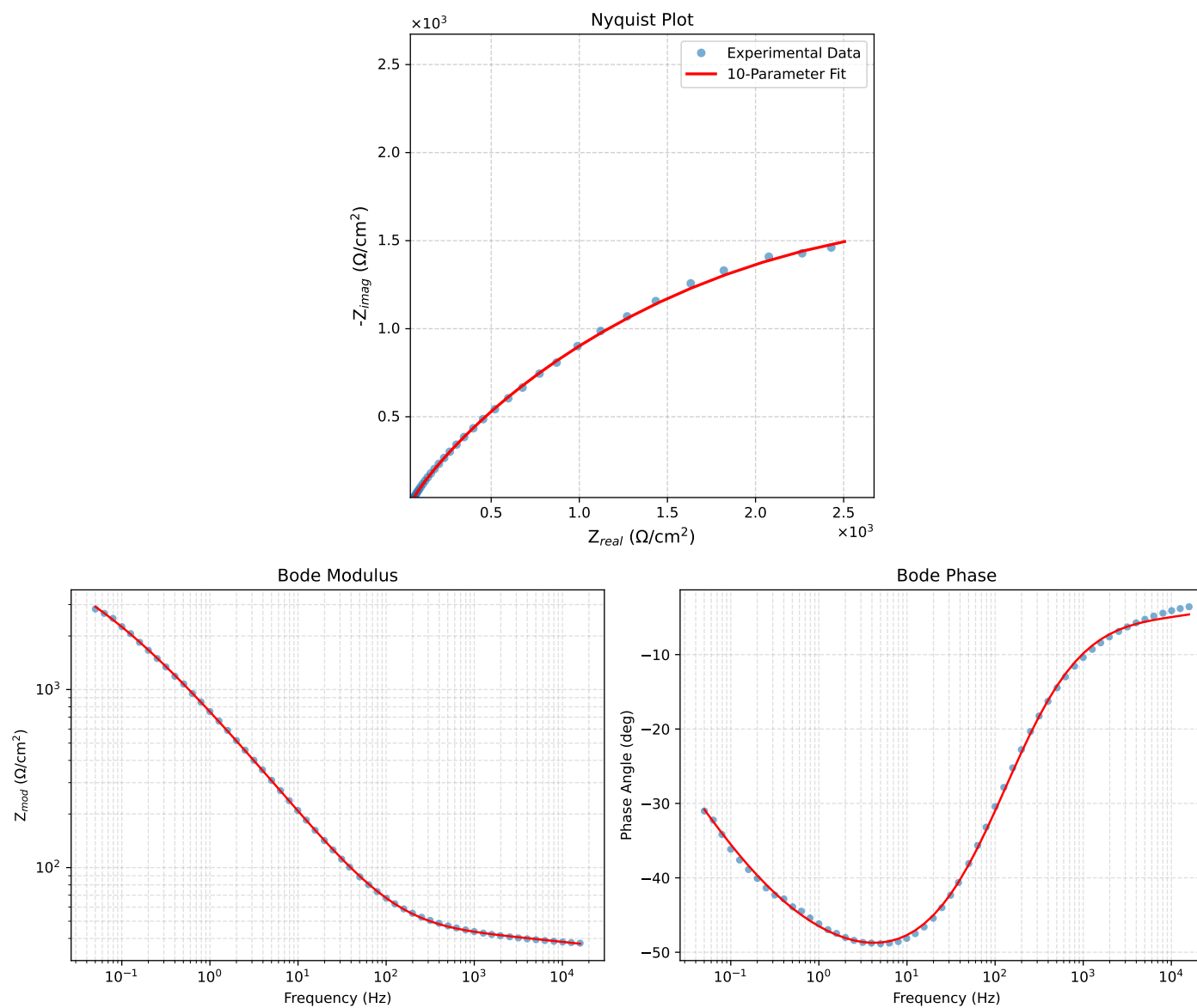
Figure 1: EIS Fit Results for Cauvel_III_NaVO3_72H
