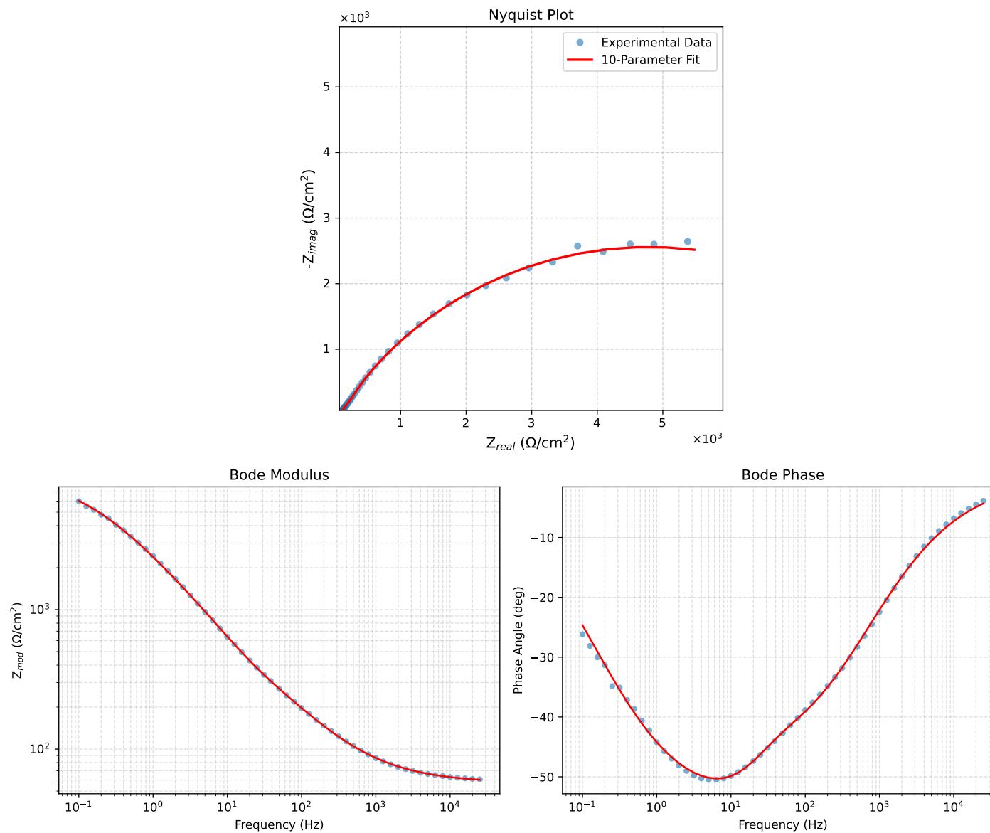
Figure 1: EIS Fit Results for CaueI.III_NaVO3_1H
