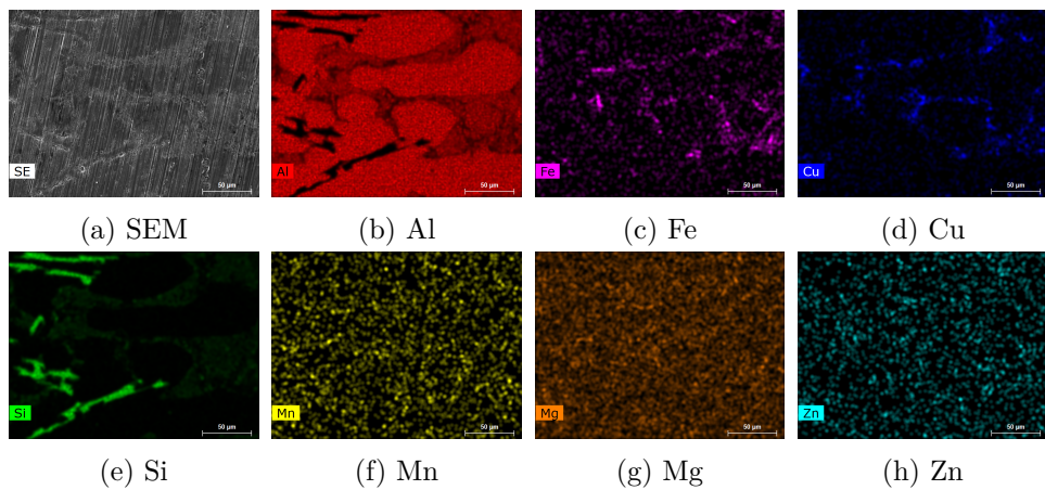
Figure 4.5: SEM-EDS of chemically etched samples.
