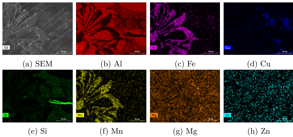
Figure 4.4: SEM-EDS of polished samples.
