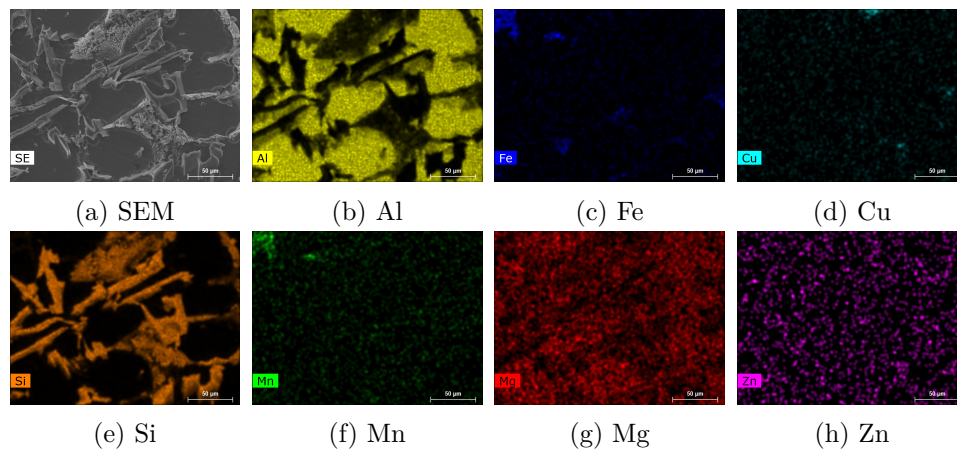
Figure 4.6: SEM-EDS of industrially etched samples.
