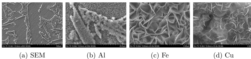
Figure 4.8: SEM-EDS of industrially etched samples.
