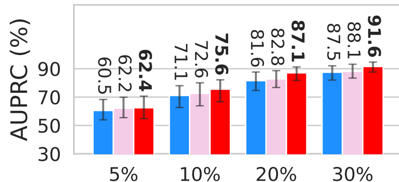
Random Forest
