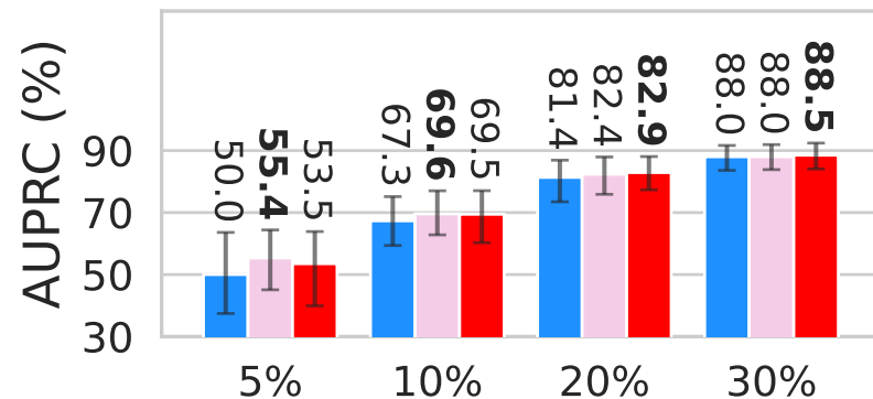
XGBoost
