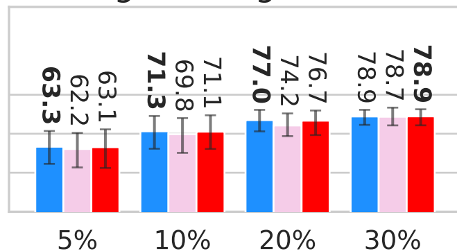
Logistic Regression
