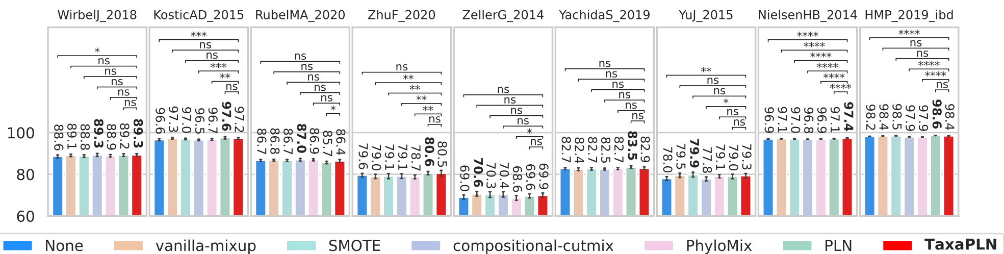
Random Forest
