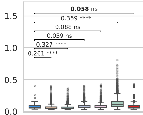
Simpson index
